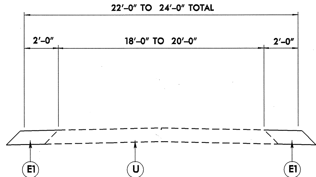
TYPICAL SECTION NO. 1
