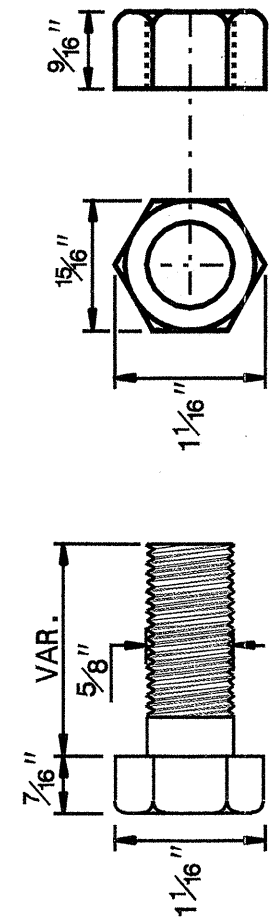
DETAIL OF STANDARD HEX BOLT AND NUT
