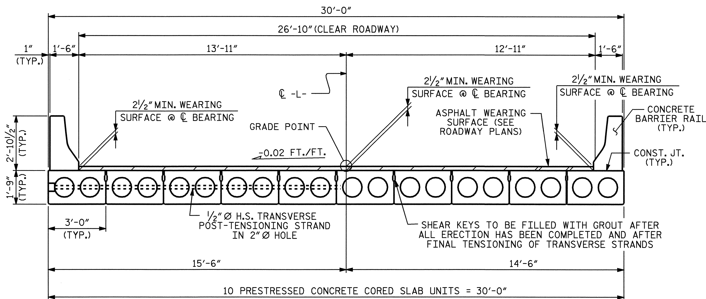
TYPICAL SECTION
