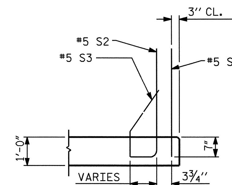
SECTION L-L
