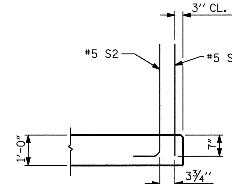
SECTION M-M
