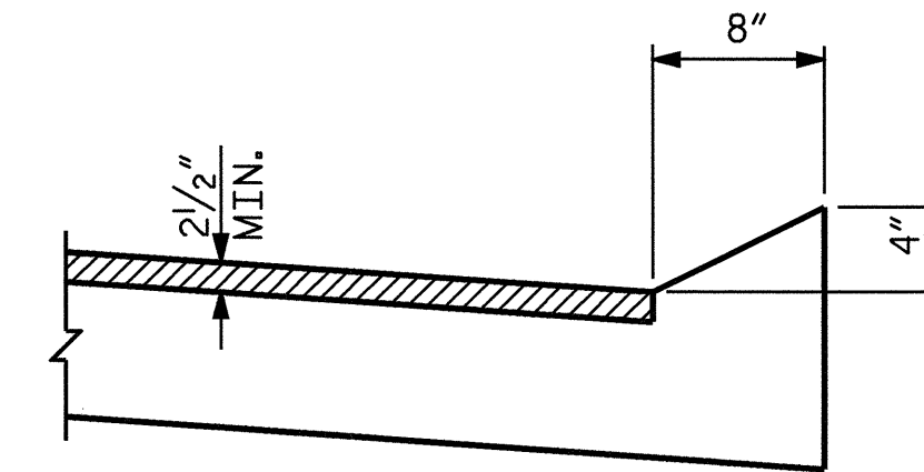
SECTION N-N
