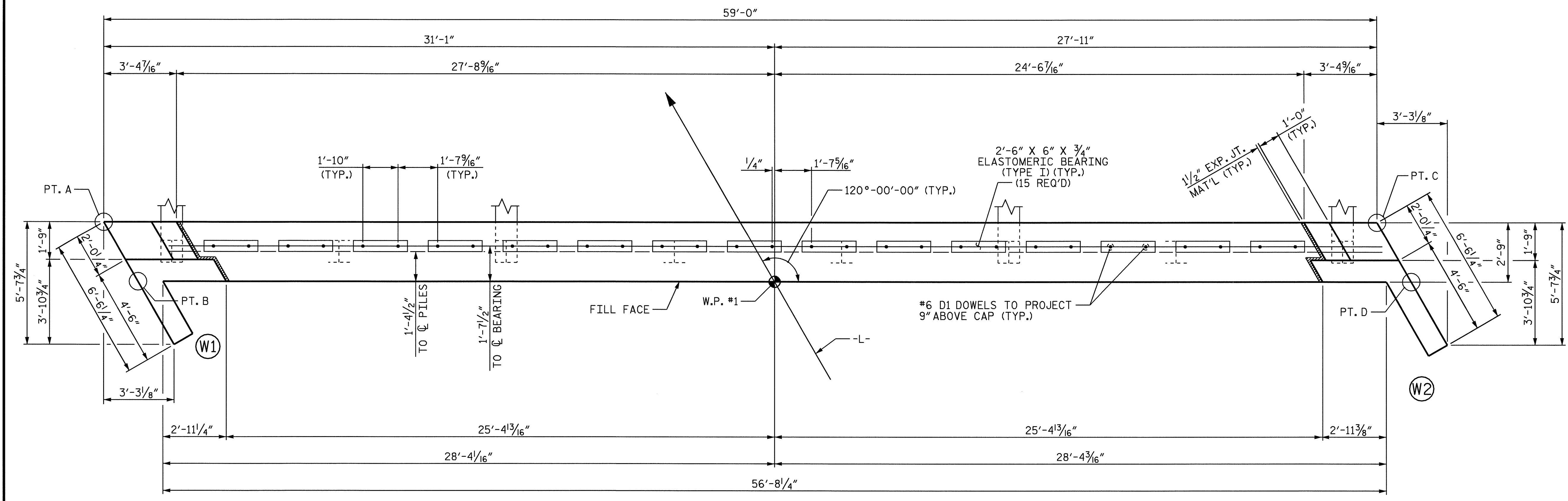
PLAN
