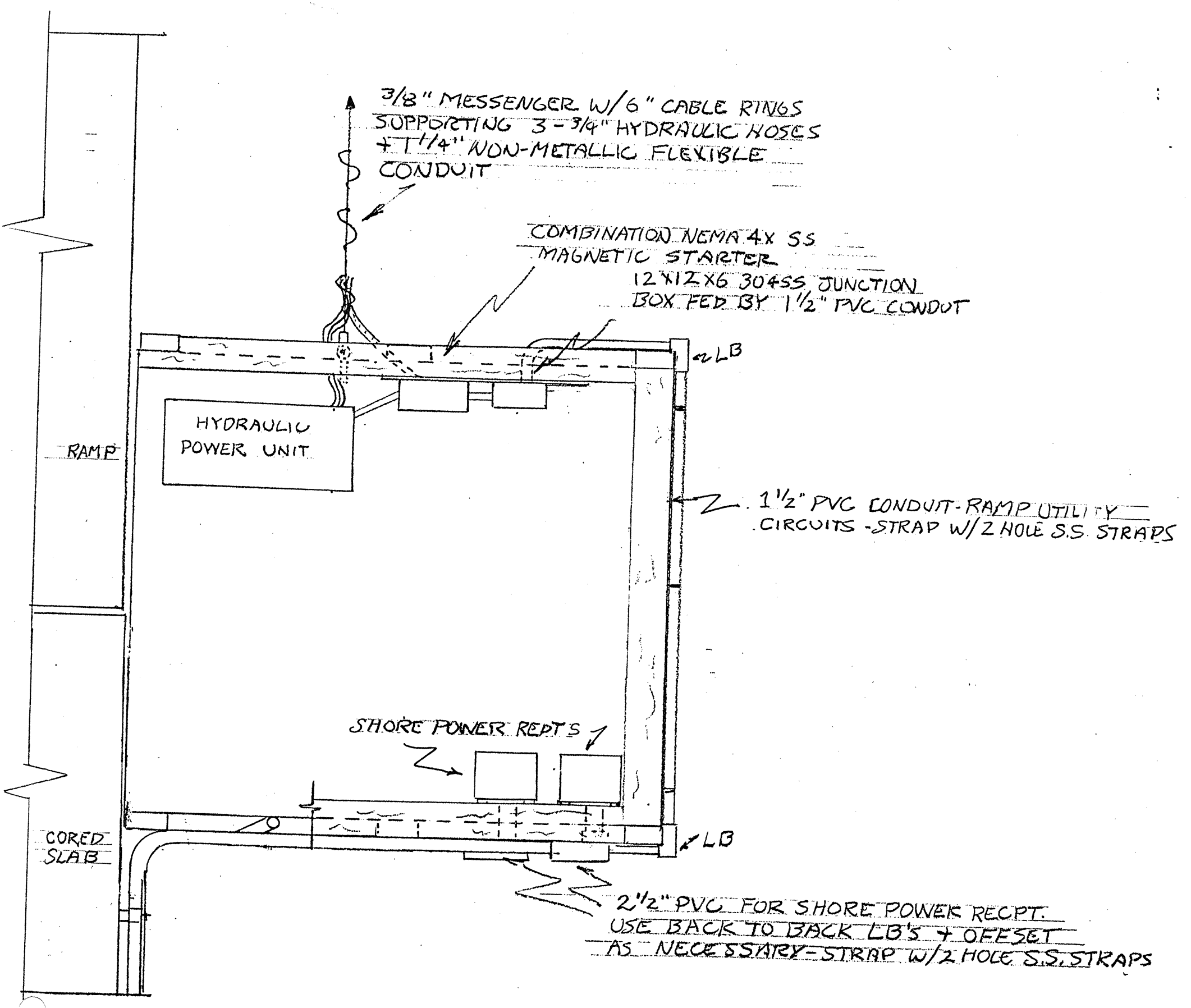
CURRITUCK HYDRAULIC PLATFORM DETAIL NOTE: KNOTTS ISLAND PLATFORM OPPOSITE HAND WITHOUT SHORE POWER RECEPTACLES
