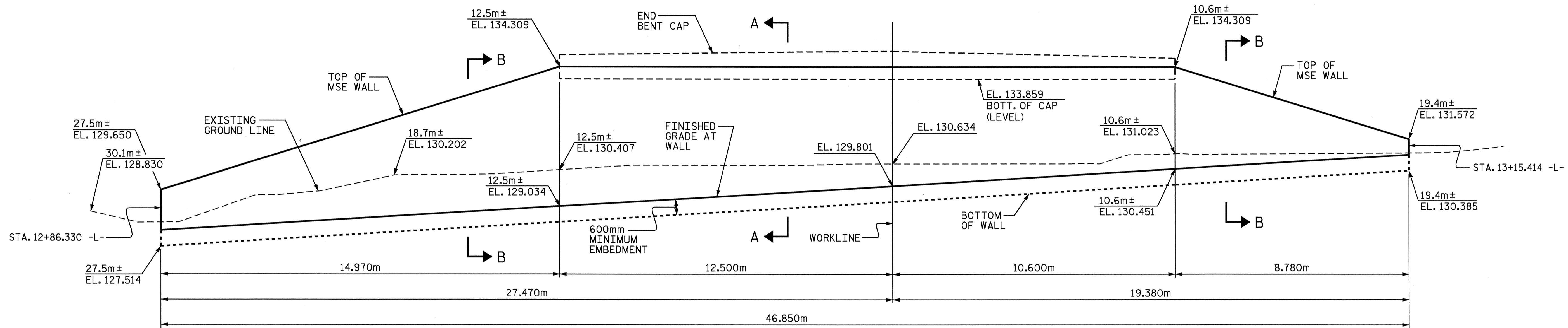
FRONT FACE OF MSE RETAINING WALL 2
