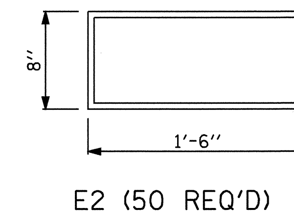
PLAN VIEW OF ELASTOMERIC BEARING
