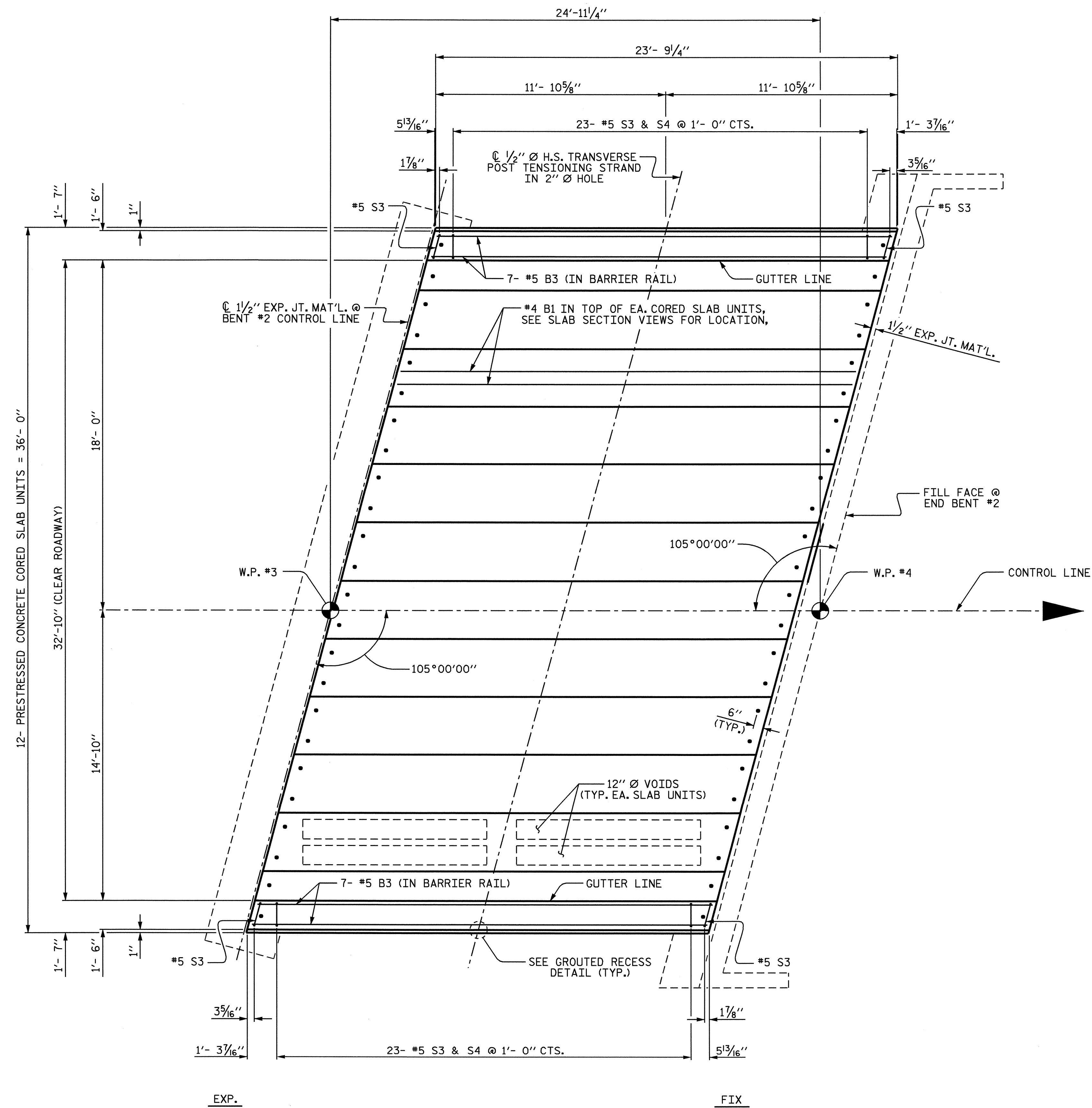
PLAN OF SPAN "C"
