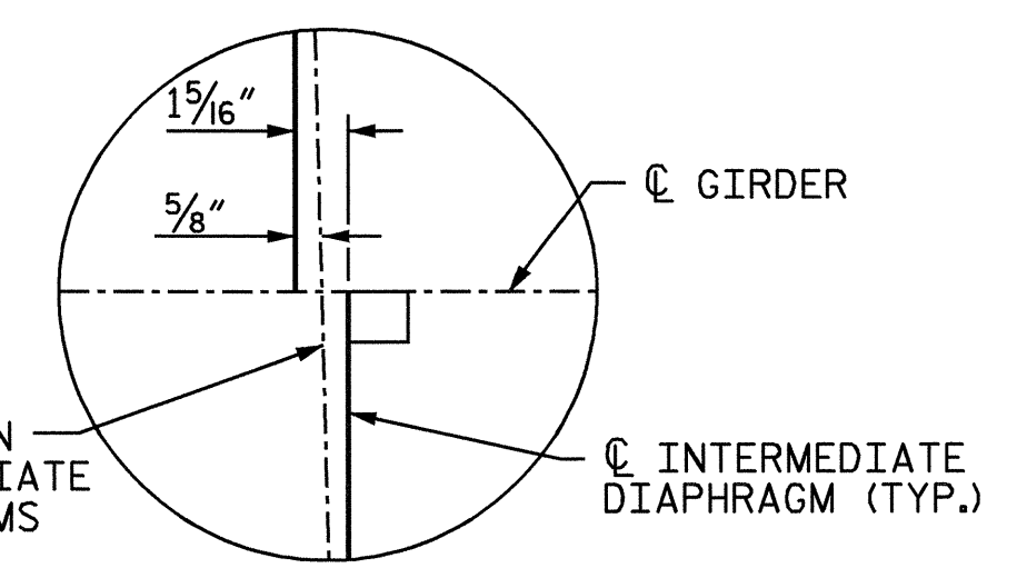
DETAIL "E" (TYPICAL EACH DIAPHRAGM AT EACH GIRDER)
