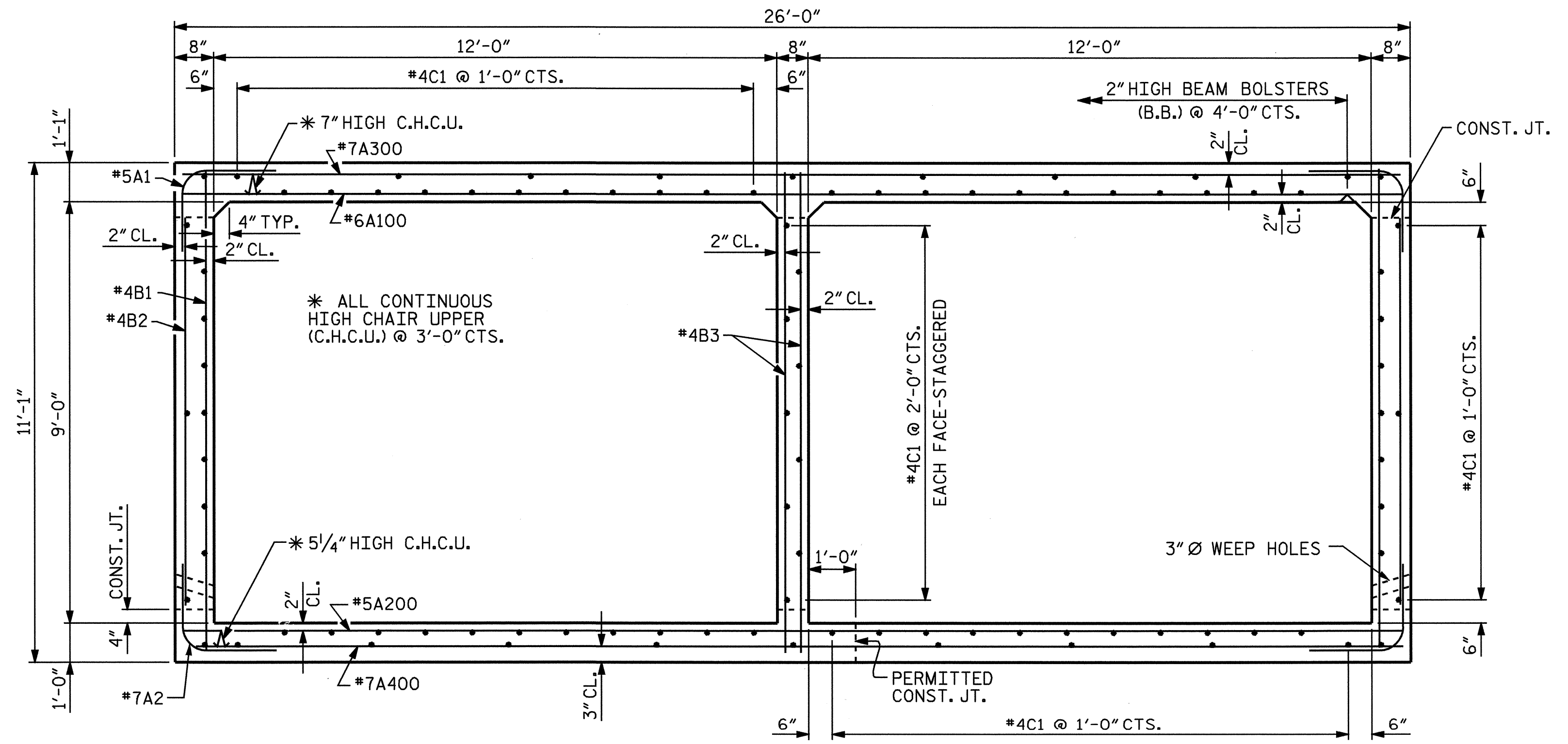
RIGHT ANGLE SECTION OF BARREL - STAGE I (THERE ARE 95 "C" BARS IN SECTION OF BARREL)
