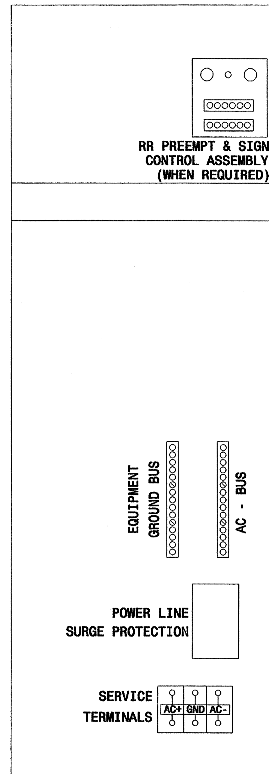
332A CABINET RIGHT SIDE
