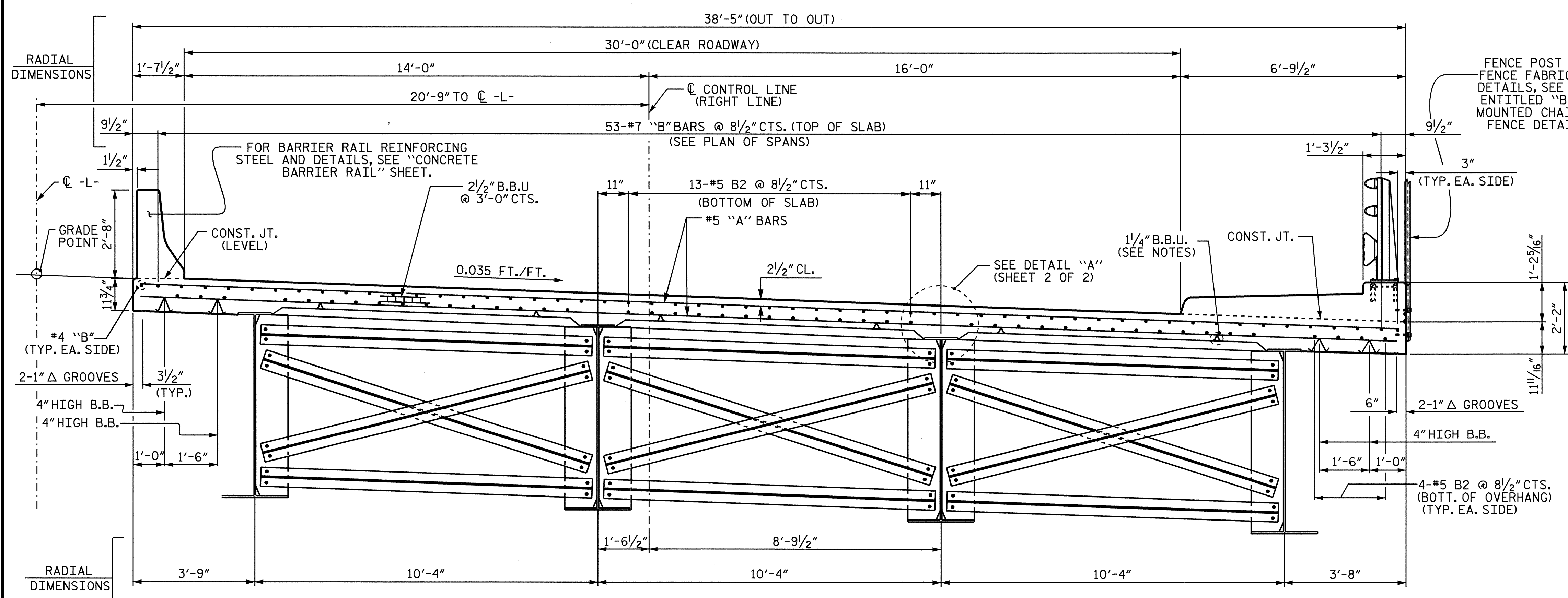
TYPICAL SECTION AT BENT AND INTERMEDIATE DIAPHRAGMS
