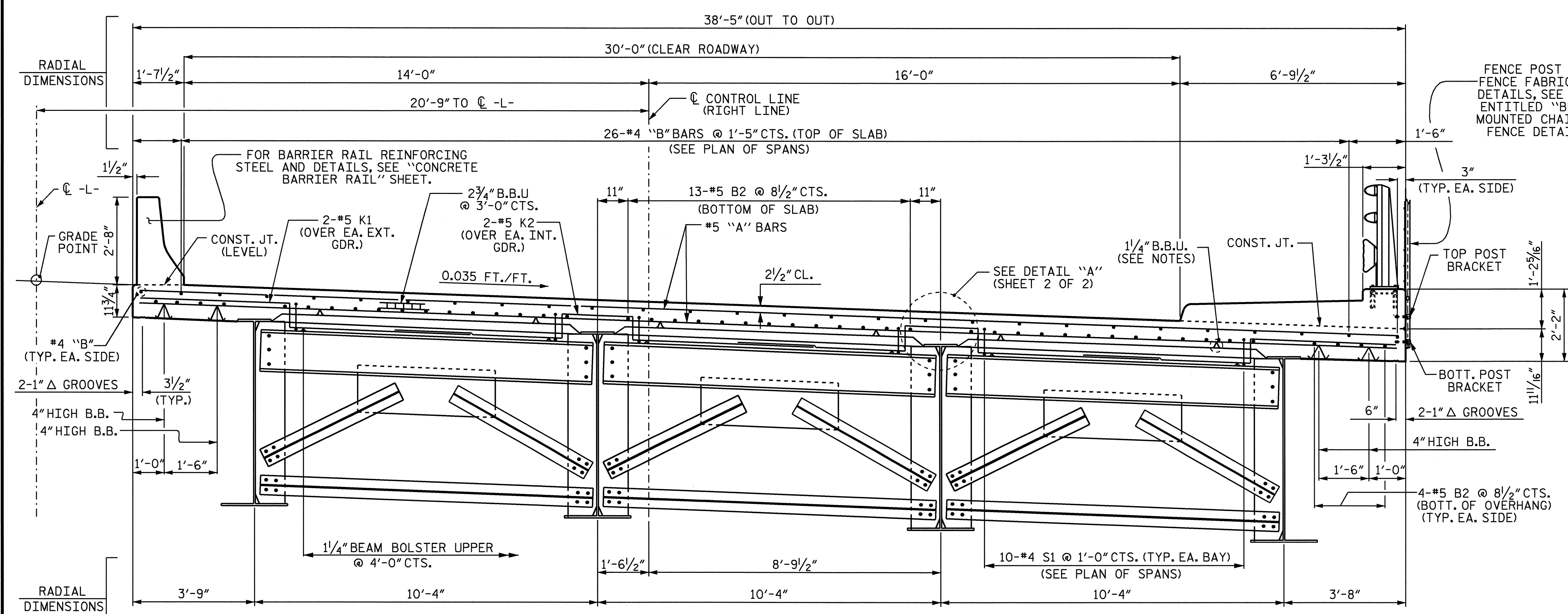
TYPICAL SECTION AT END BENT
