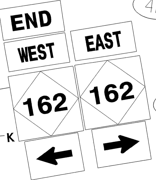
PROPOSED SIGNS STA. 21+00 TO STA. 32+00 HOPE MILLS BYPASS
