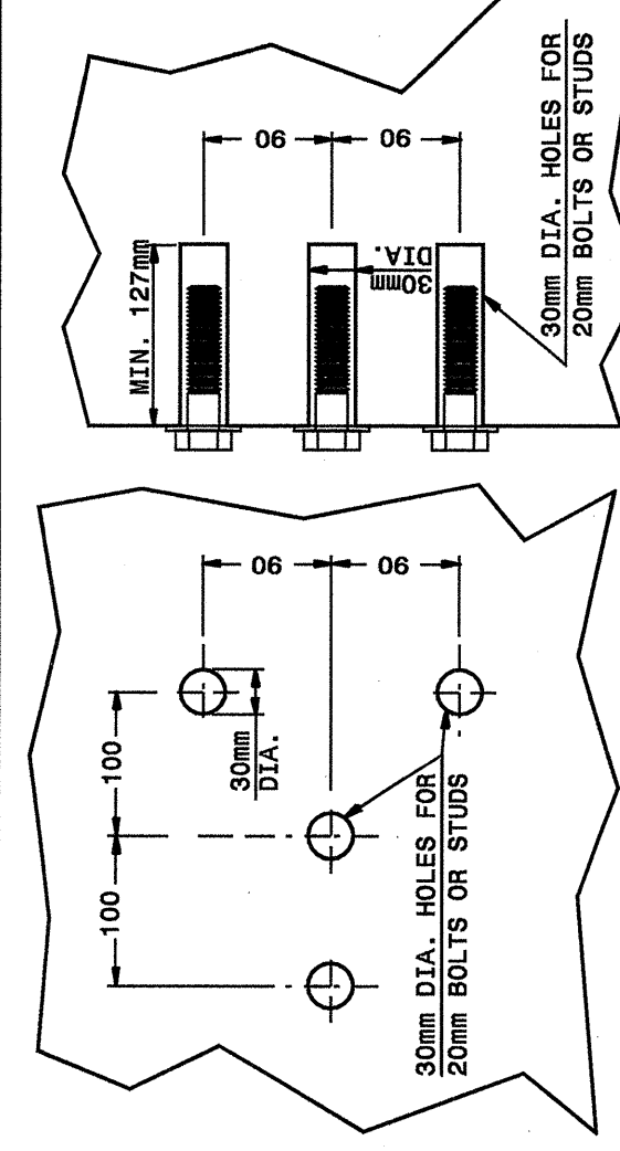
DETAIL B
