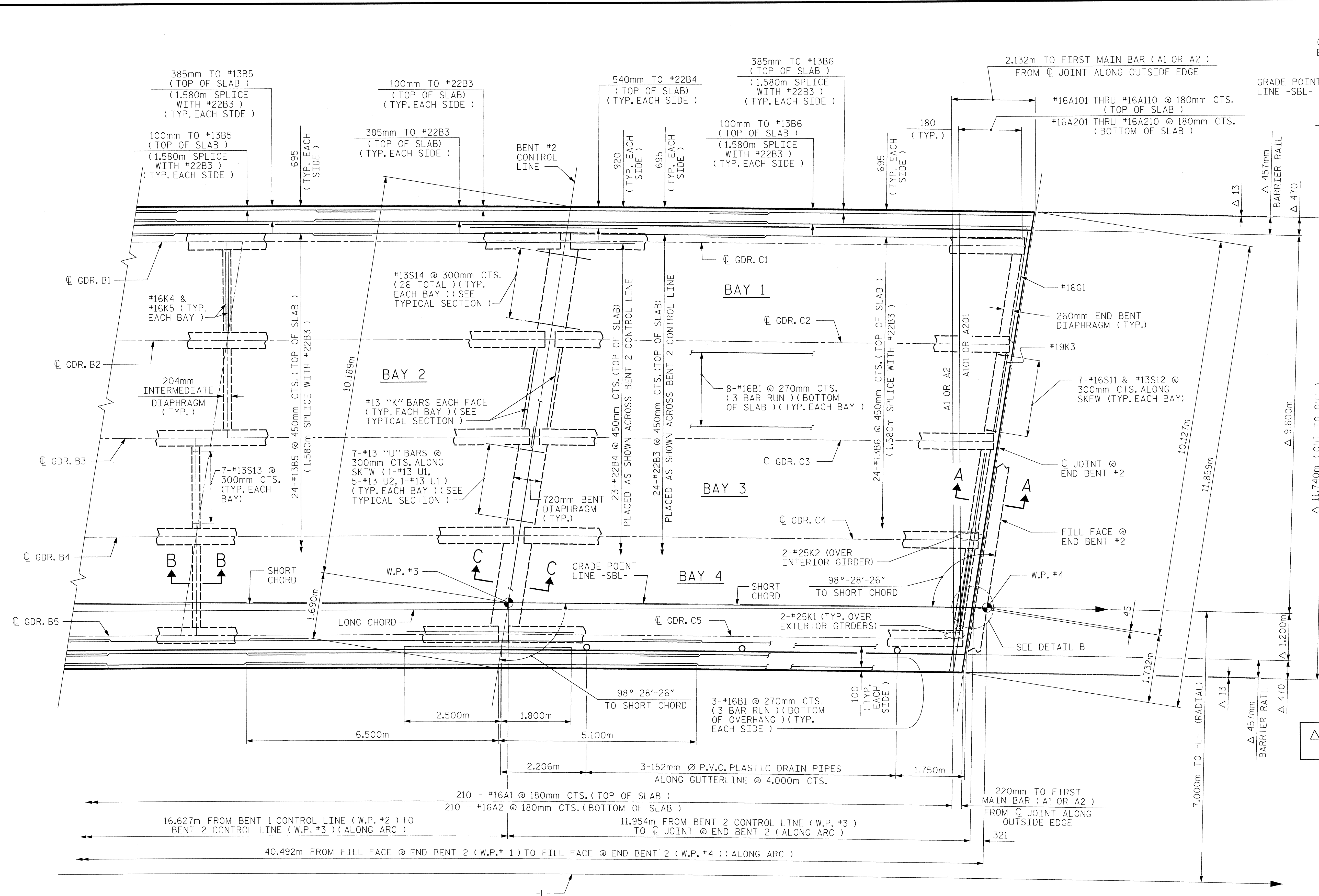
PLAN OF SPAN B - PARTIAL
