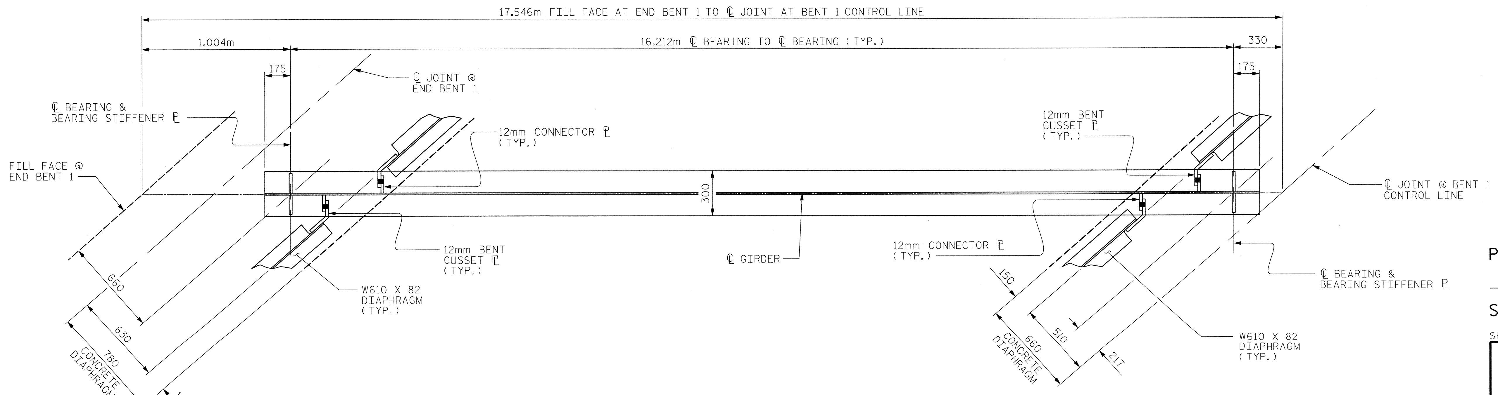
BOTTOM FLANGE DETAILS ( SEE TOP FLANGE CLIP DETAILS, SHEET 5 OF 6 )
