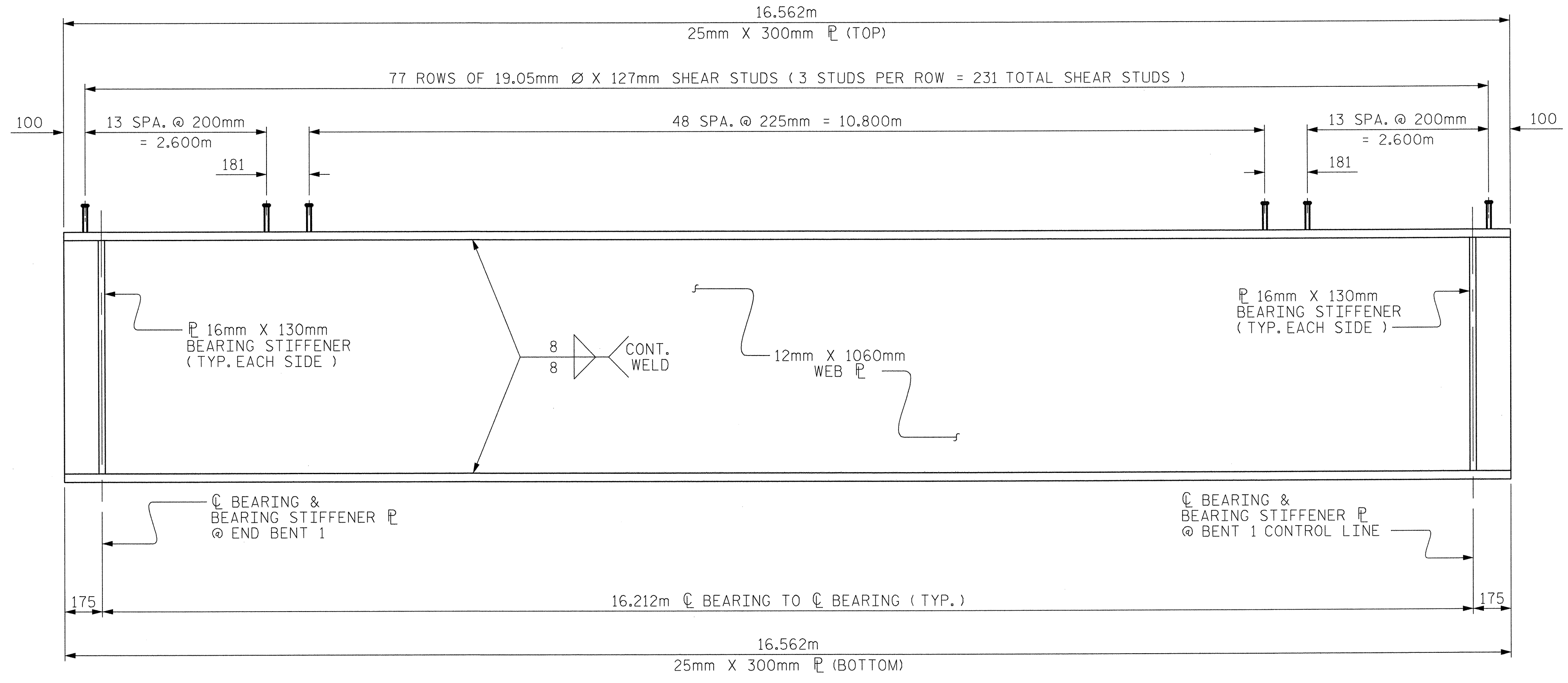
GIRDER ELEVATION ( CONNECTOR PLATES OMITTED FOR CLARITY )
