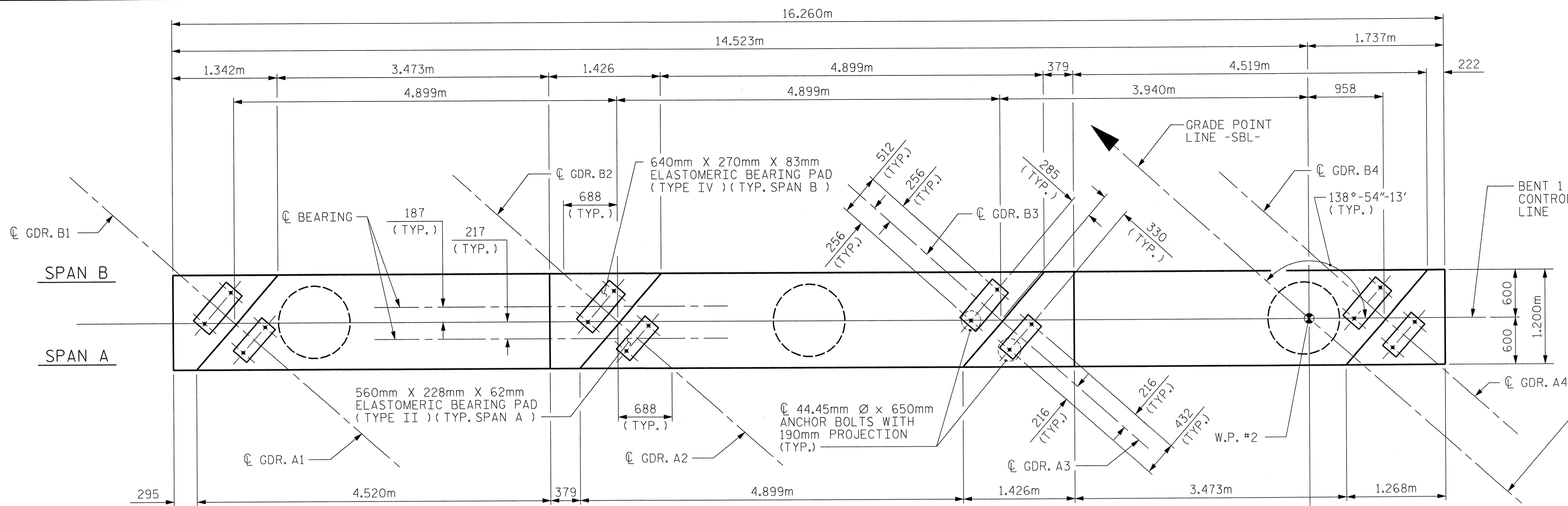
PLAN
