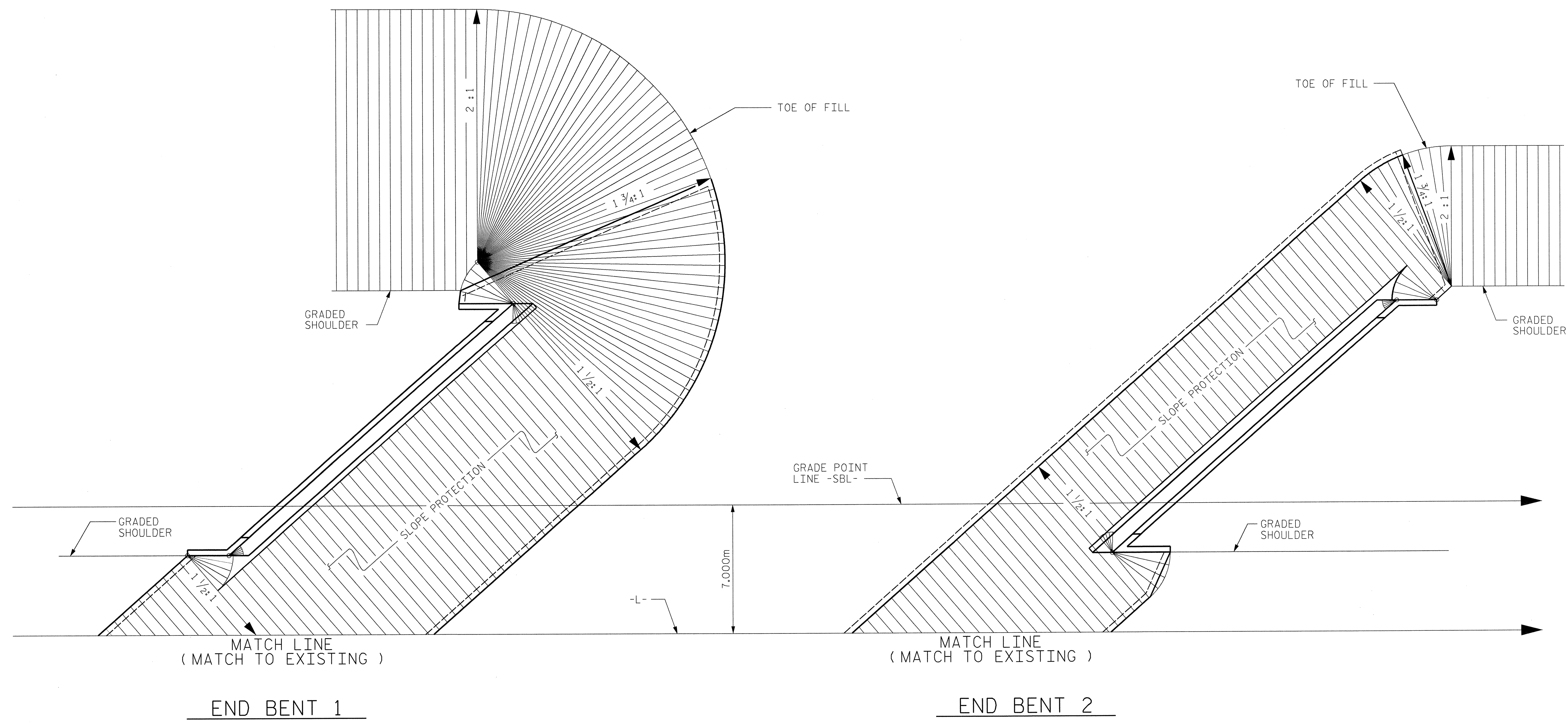
PLAN - END BENT WITH SWEEPED BACK WINGS - SKEWED (1 1/2:1 SLOPE)
