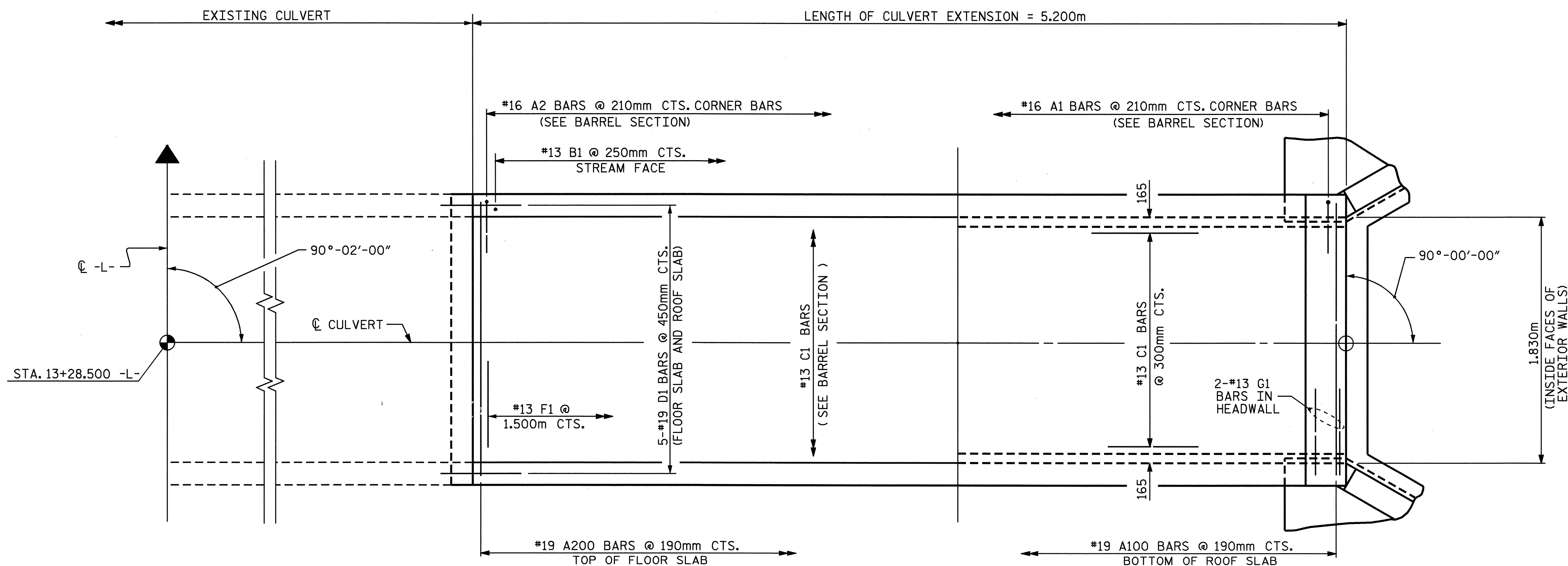
PART PLAN - FLOOR SLAB
