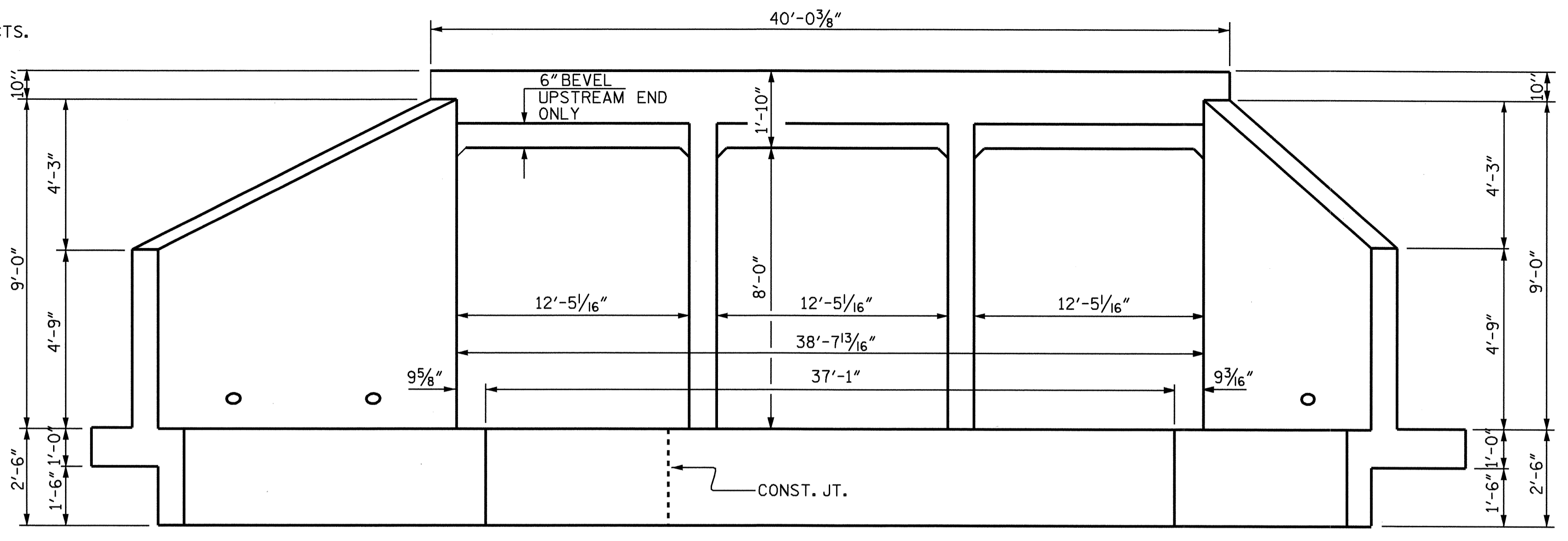
END ELEVATION NORMAL TO SKEW (LOOKING DOWNSTREAM)
