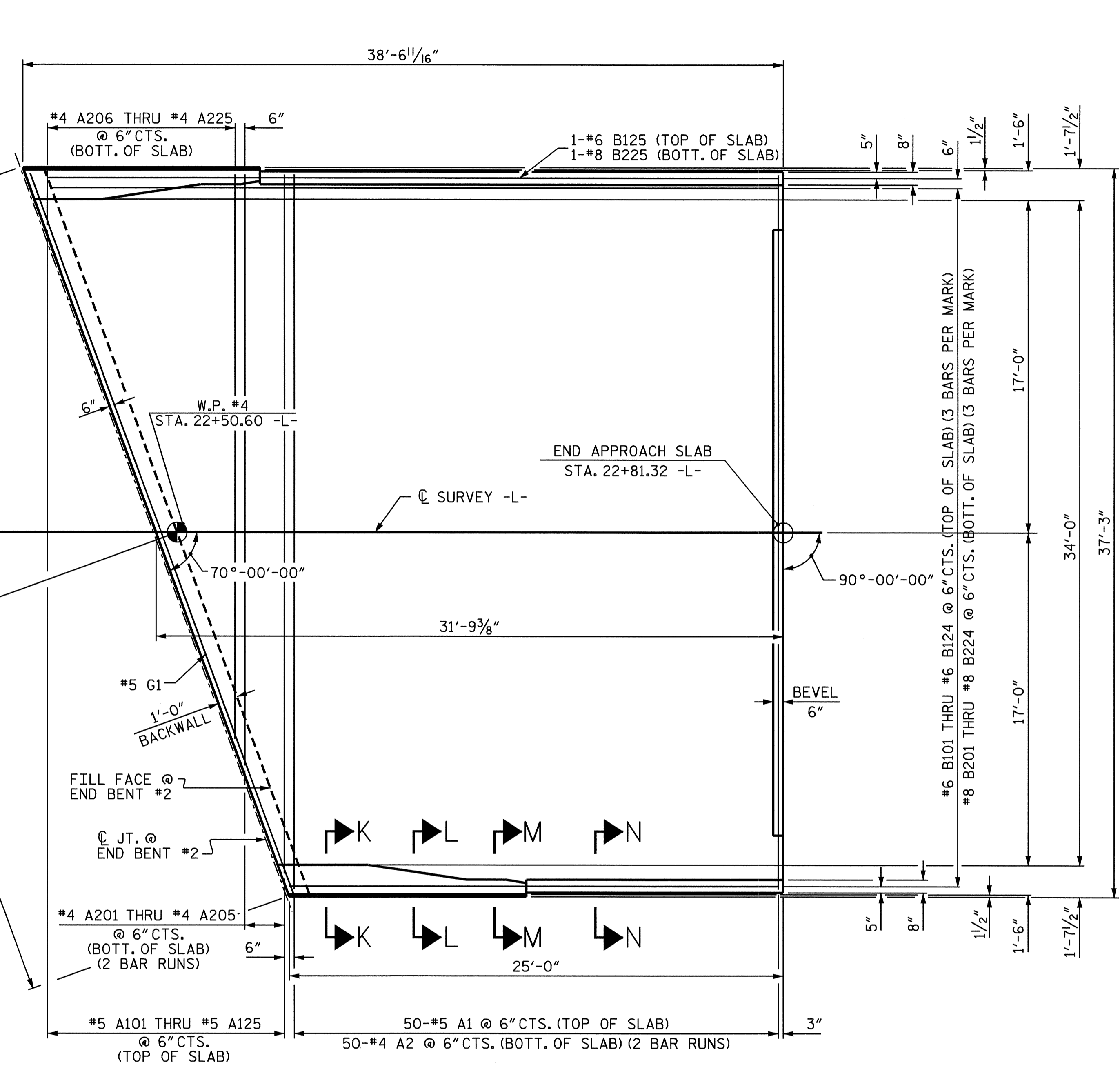
PLAN OF APPROACH SLAB @ END BENT #2
