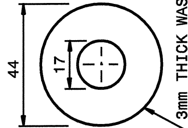
DETAIL OF STANDARD WASHER
