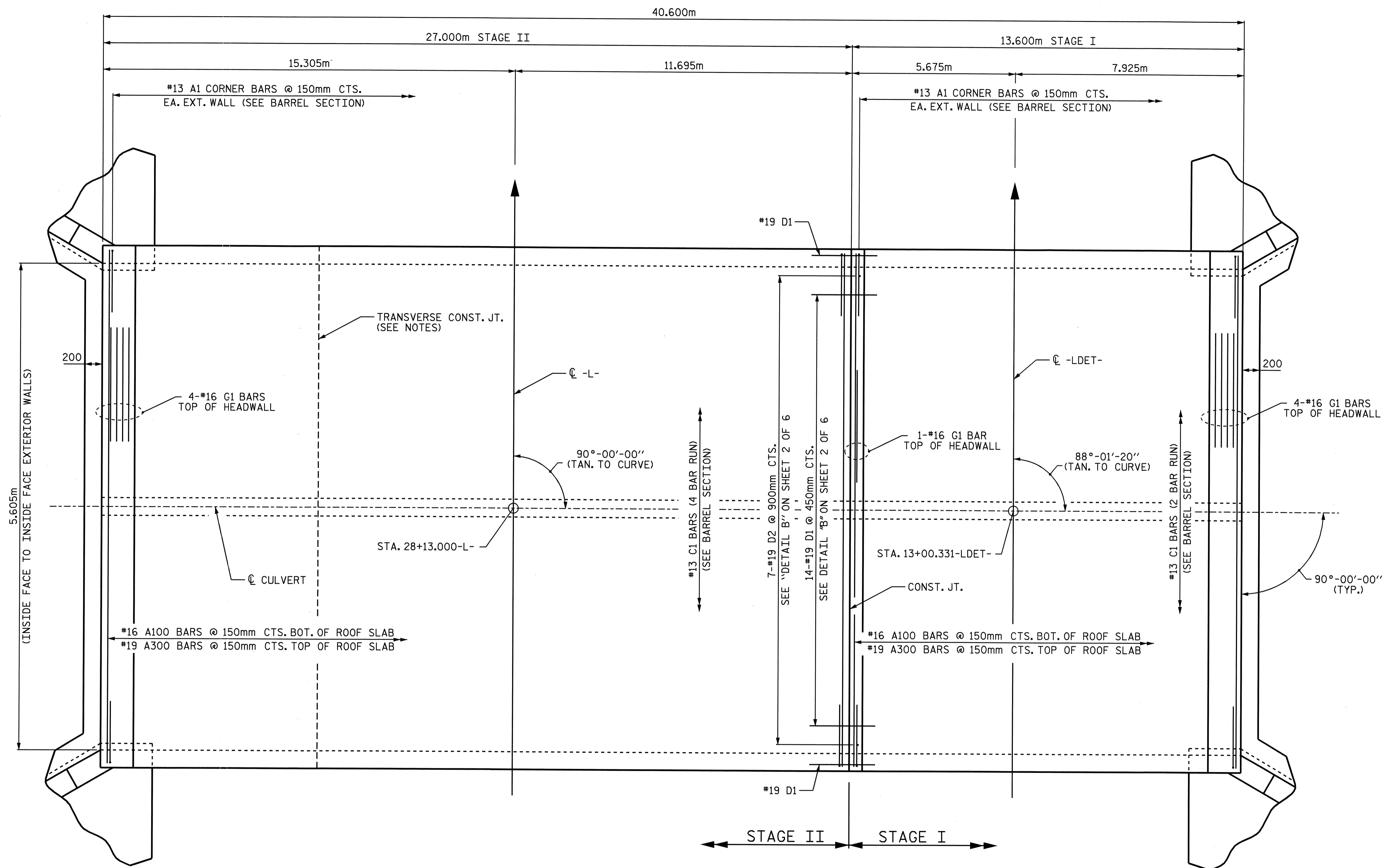
PLAN OF ROOF SLAB
