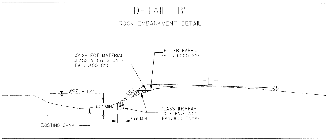
FROM STA. 29+25 -L- TO 31+25 -L- LT.
