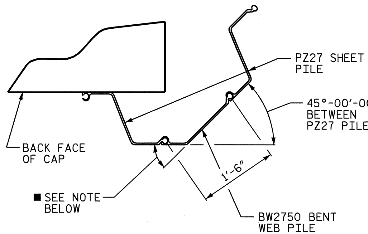
DETAIL "B"
