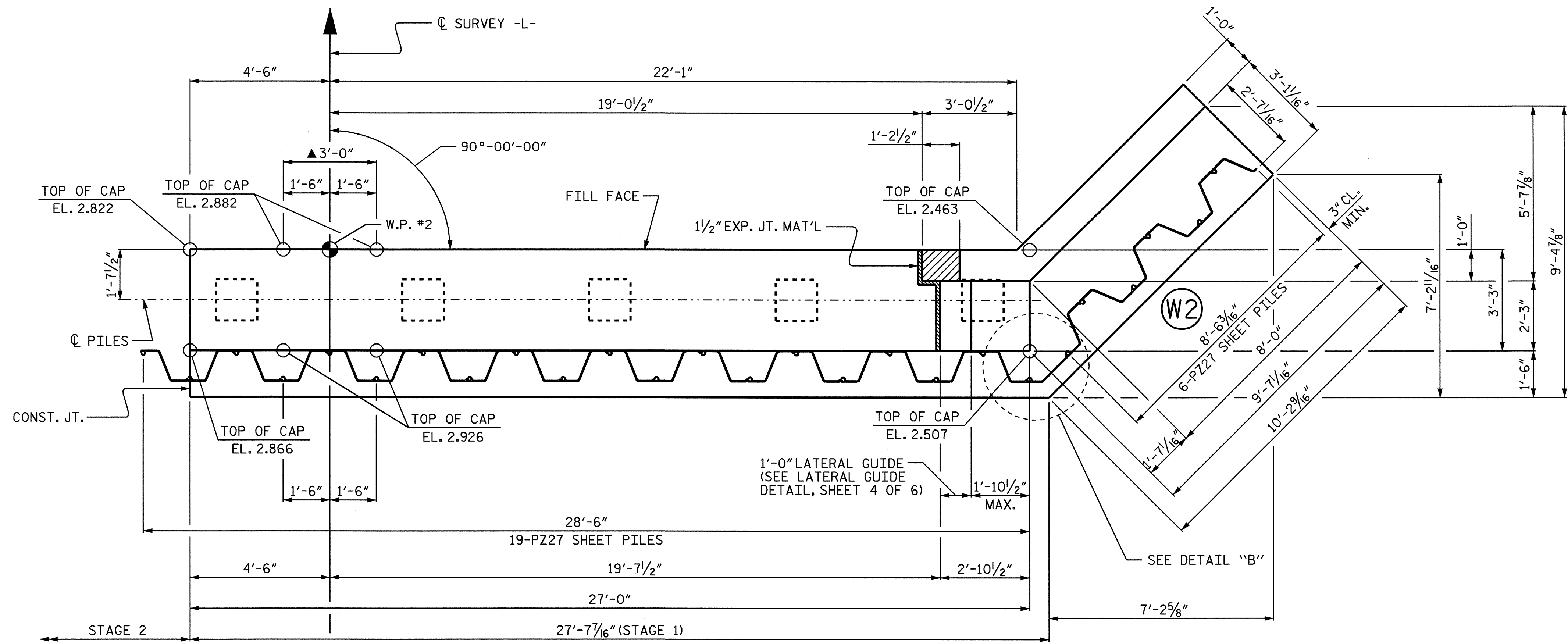
PLAN (STAGE 1)
