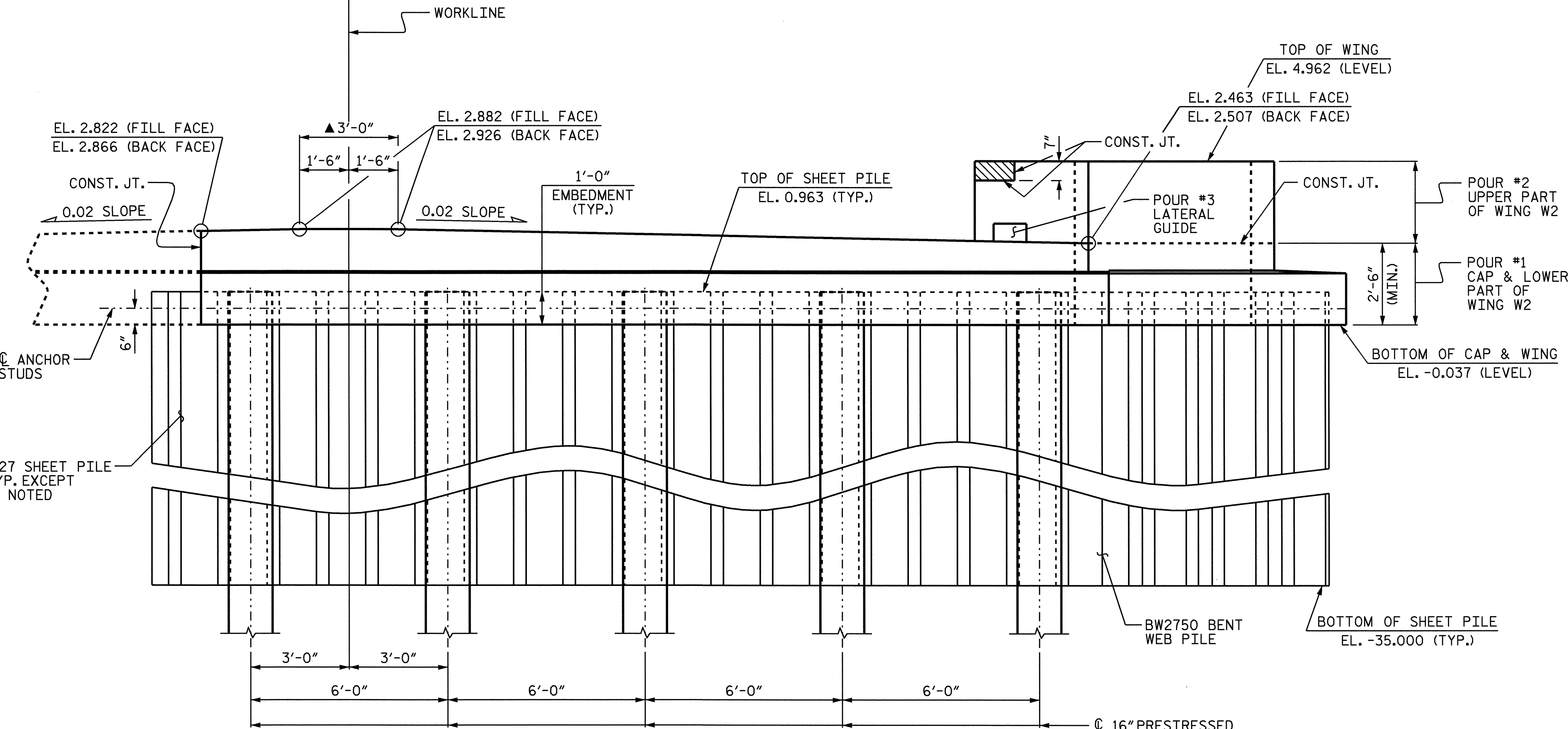
ELEVATION (STAGE 1)
