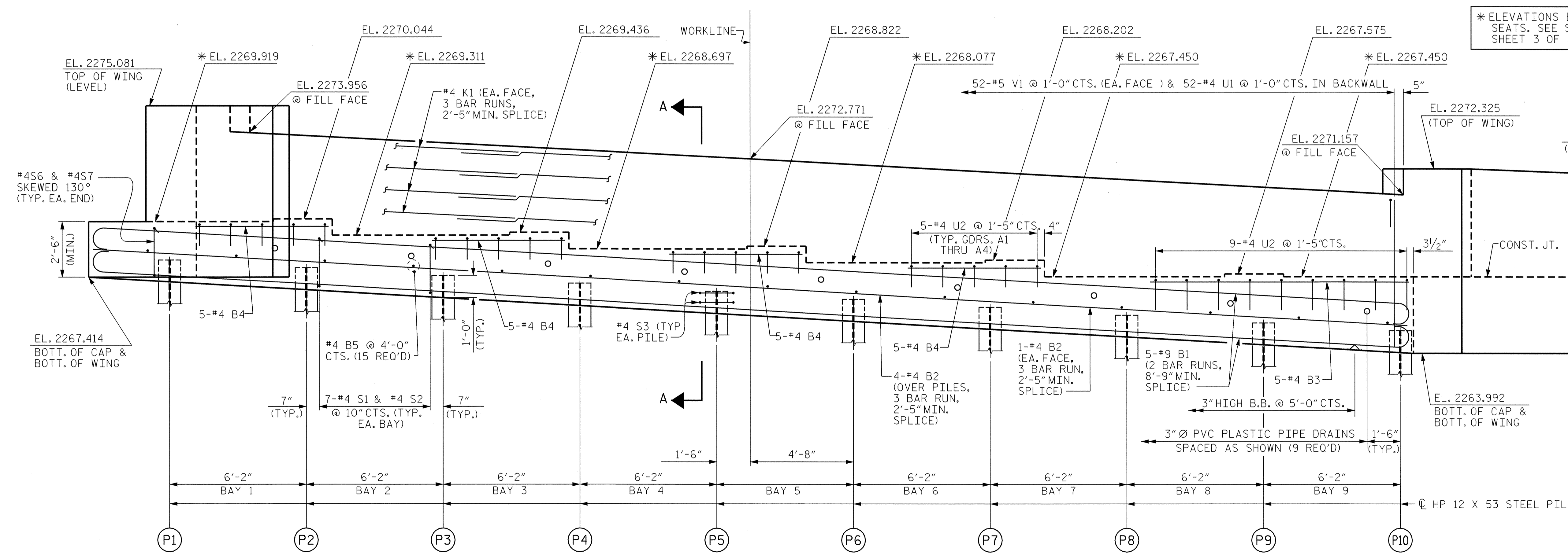
ELEVATION WING PILE NOT SHOWN
