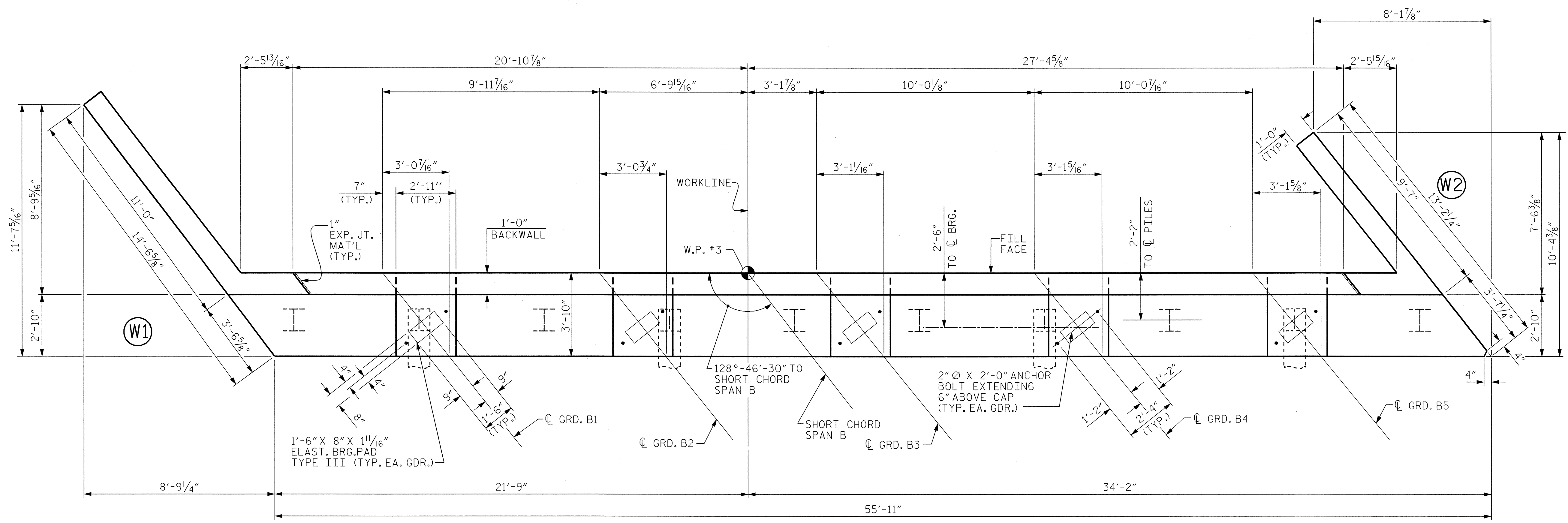
PLAN
