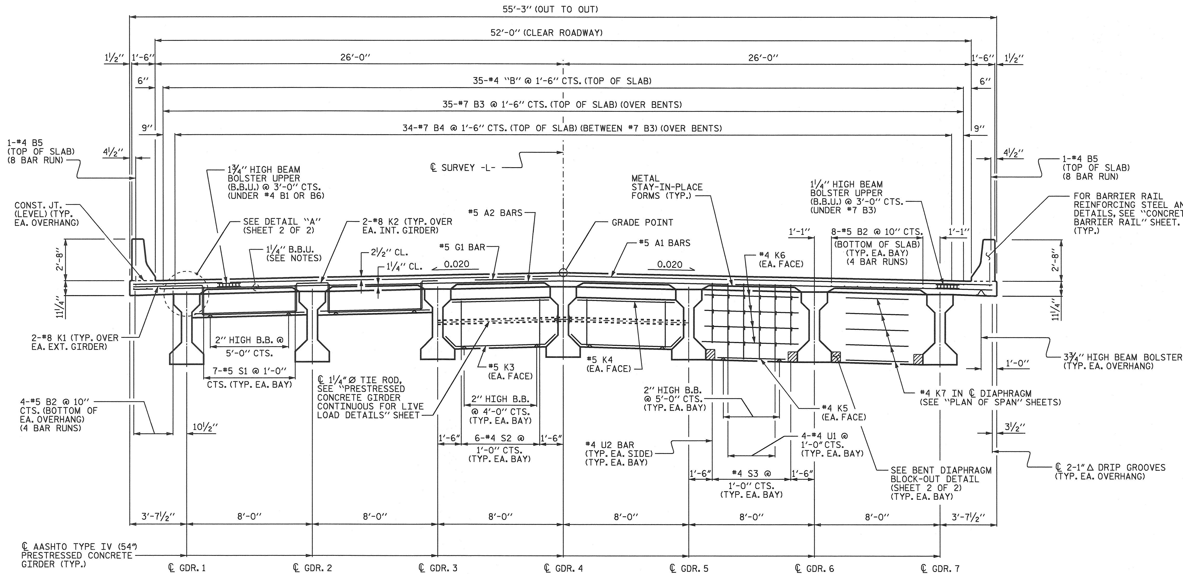
PARTIAL TYPICAL SECTION (SHOWING END BENT DIAPHRAGMS)
