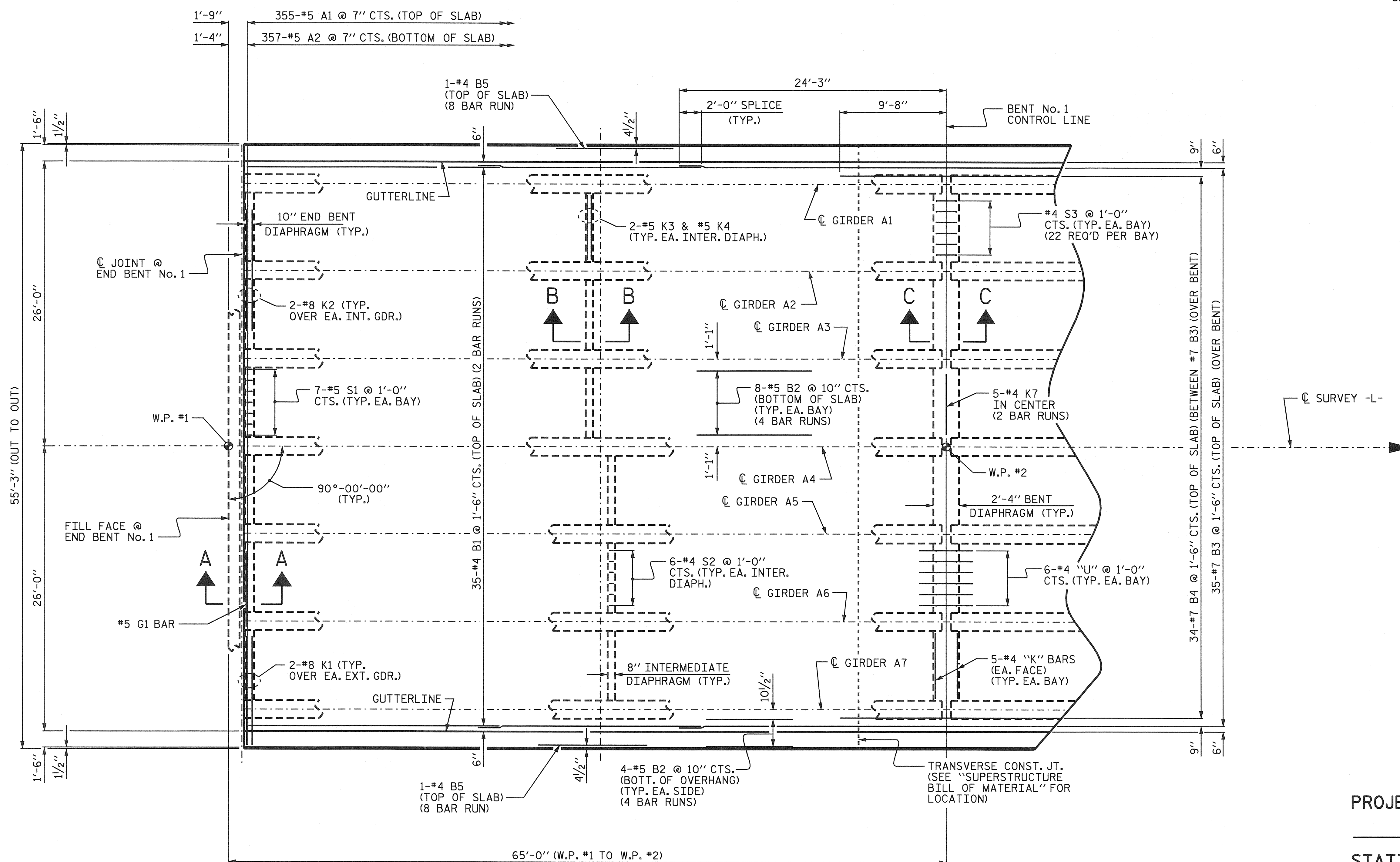
PLAN OF SPAN "A"
