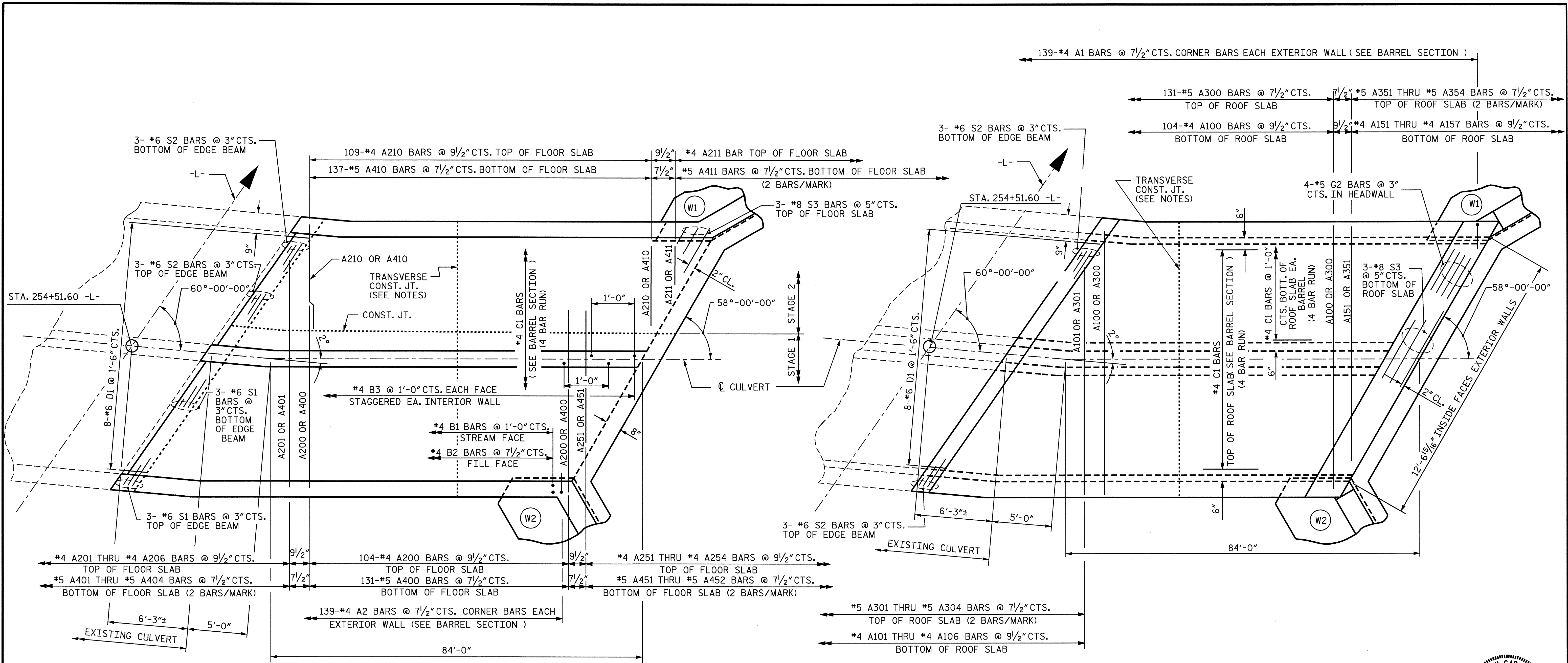
EXTENSION - FLOOR SLAB
