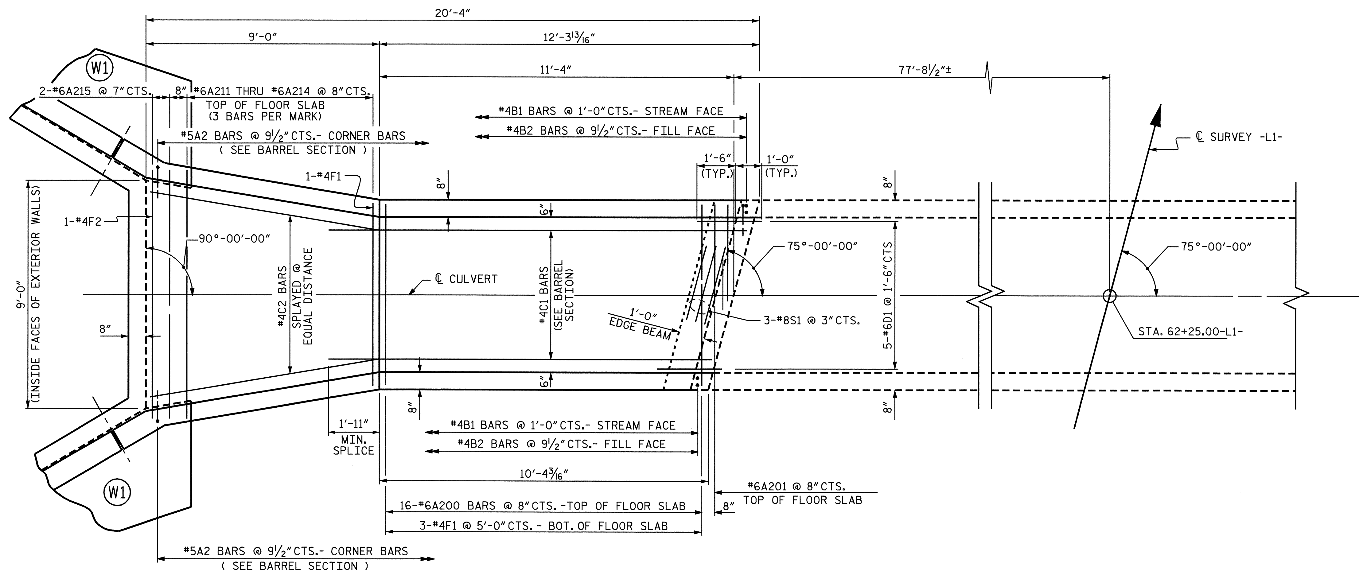
FLOOR SLAB LEFT EXTENSION
