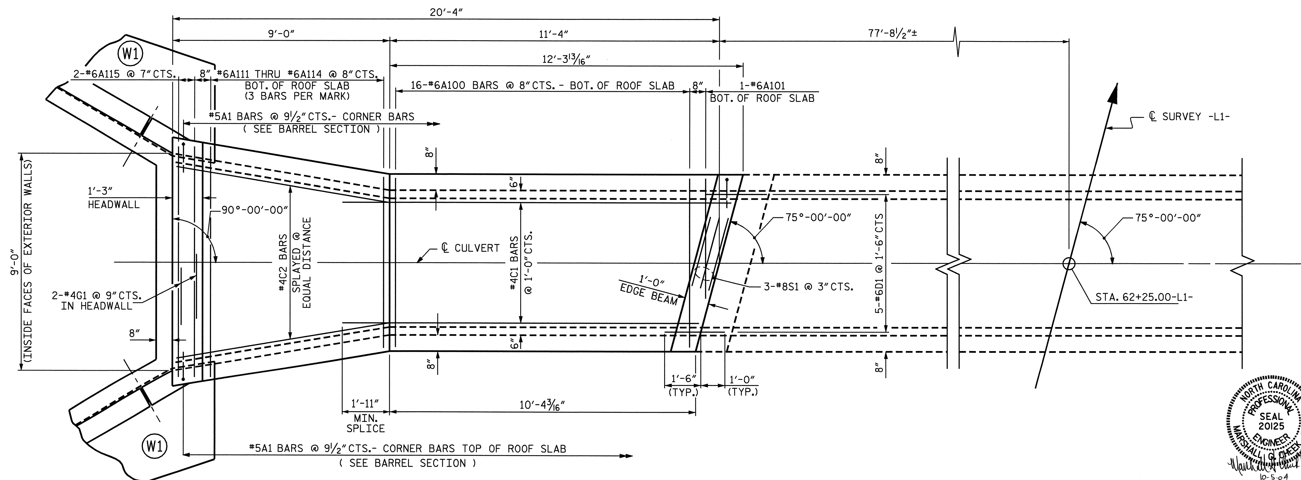
ROOF SLAB LEFT EXTENSION
