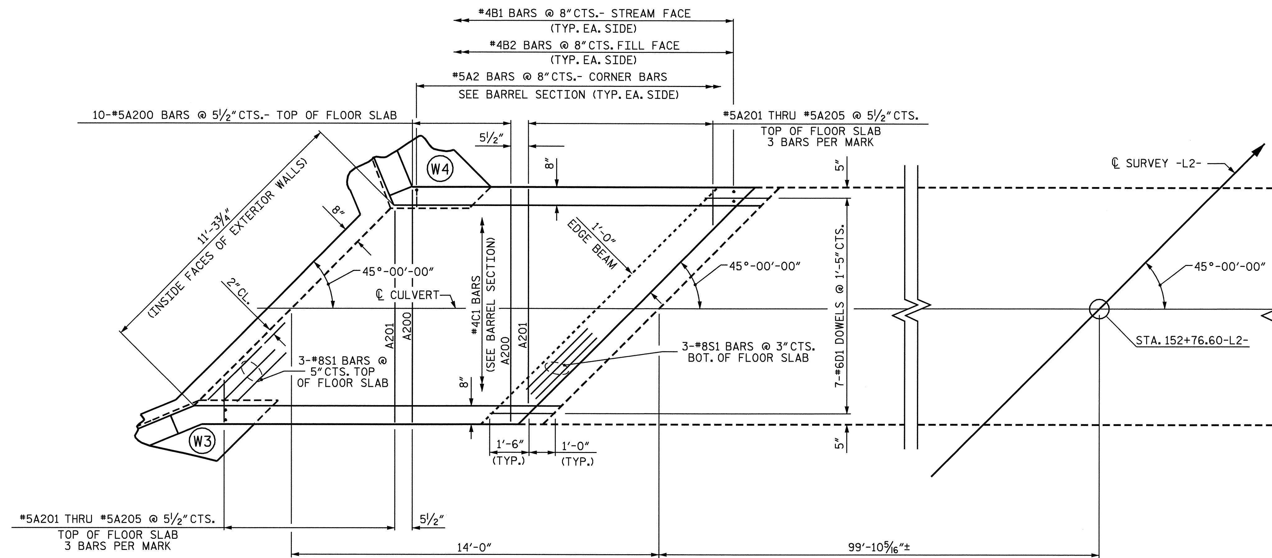
FLOOR SLAB LEFT EXTENSION
