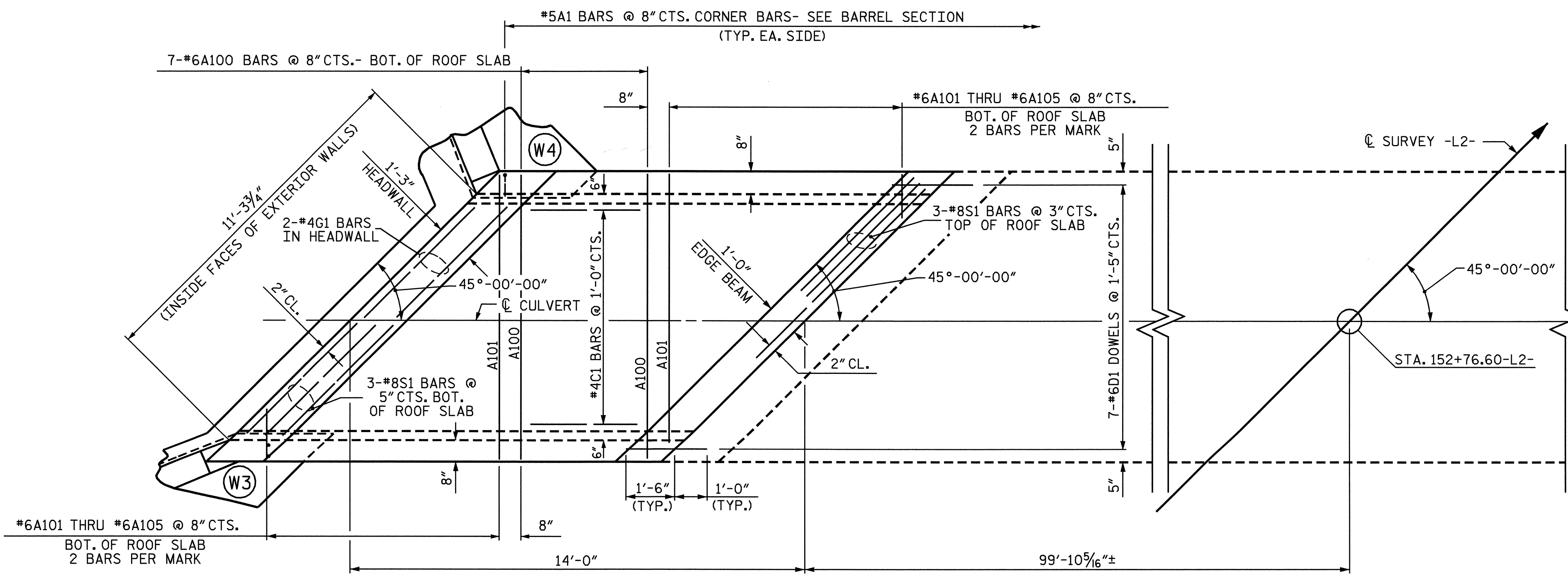
ROOF SLAB LEFT EXTENSION
