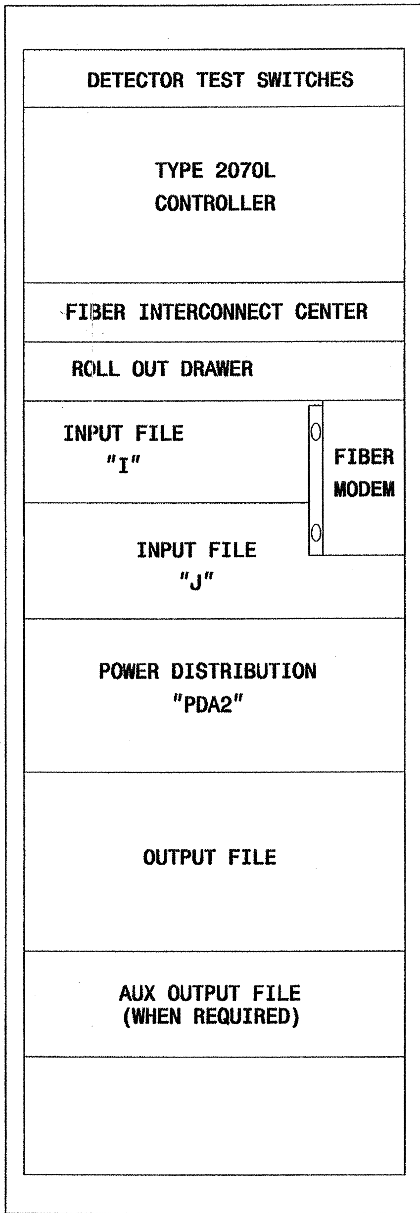
332A CABINET
