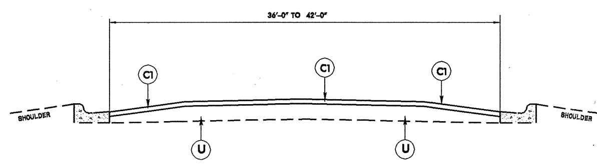
TYPICAL SECTION NO. 3 ** NOTE: USE ON MAP 3
