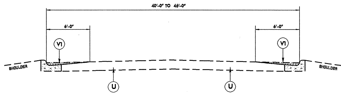
TYPICAL SECTION NO. 1 ** NOTE: USE ON MAP 3
