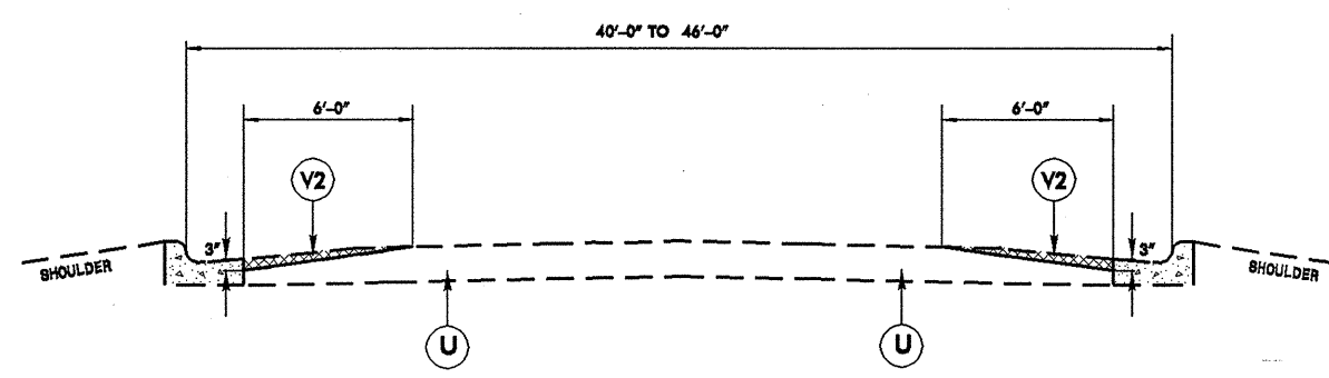
TYPICAL SECTION NO. 2 ** NOTE: USE ON MAP 3
