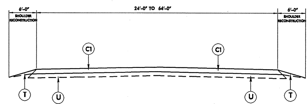
TYPICAL SECTION NO. 5 ** NOTE: USE ON MAPS 1, 2, 4, 5
