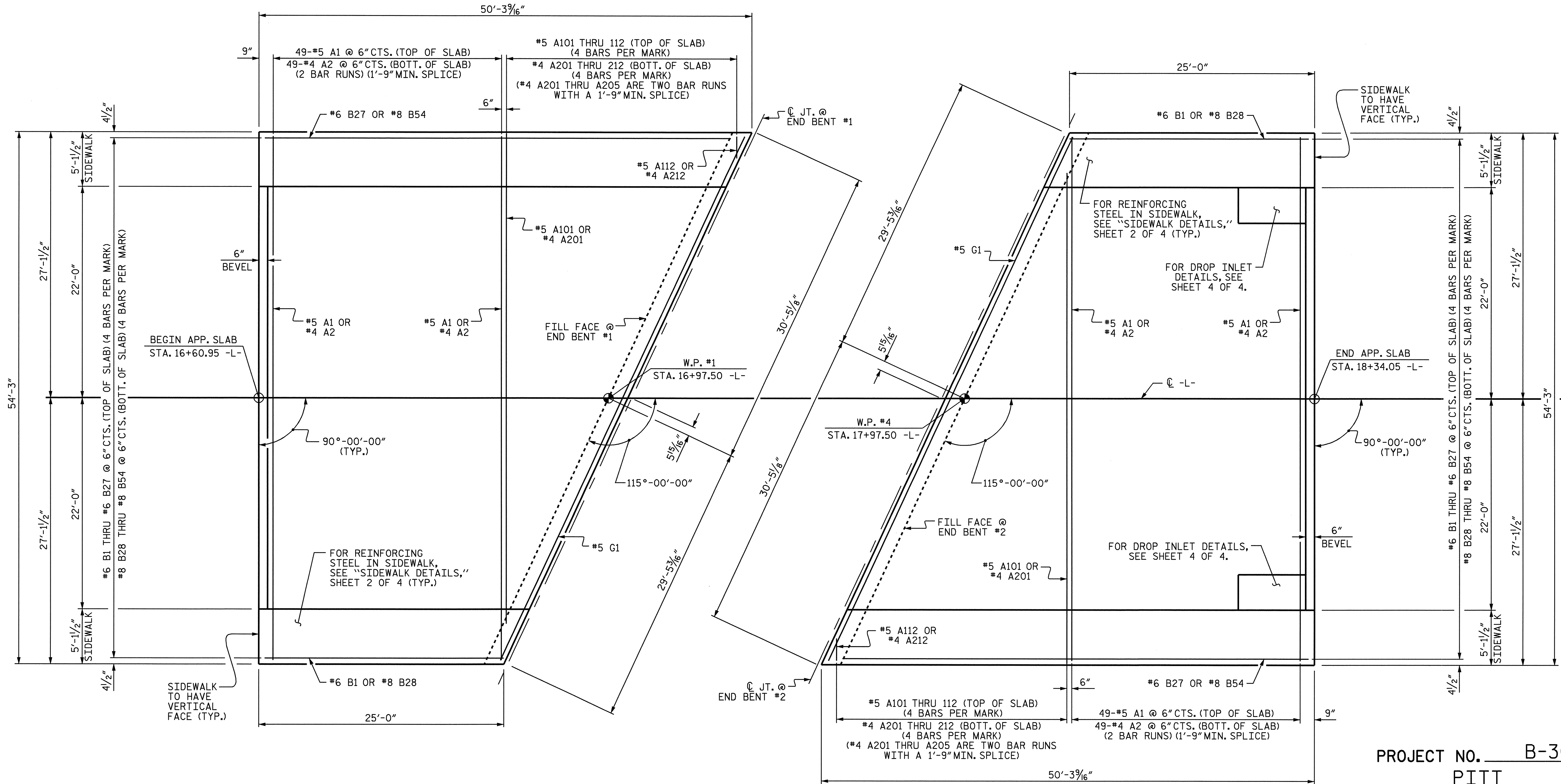
APPROACH SLAB @ END BENT #1
