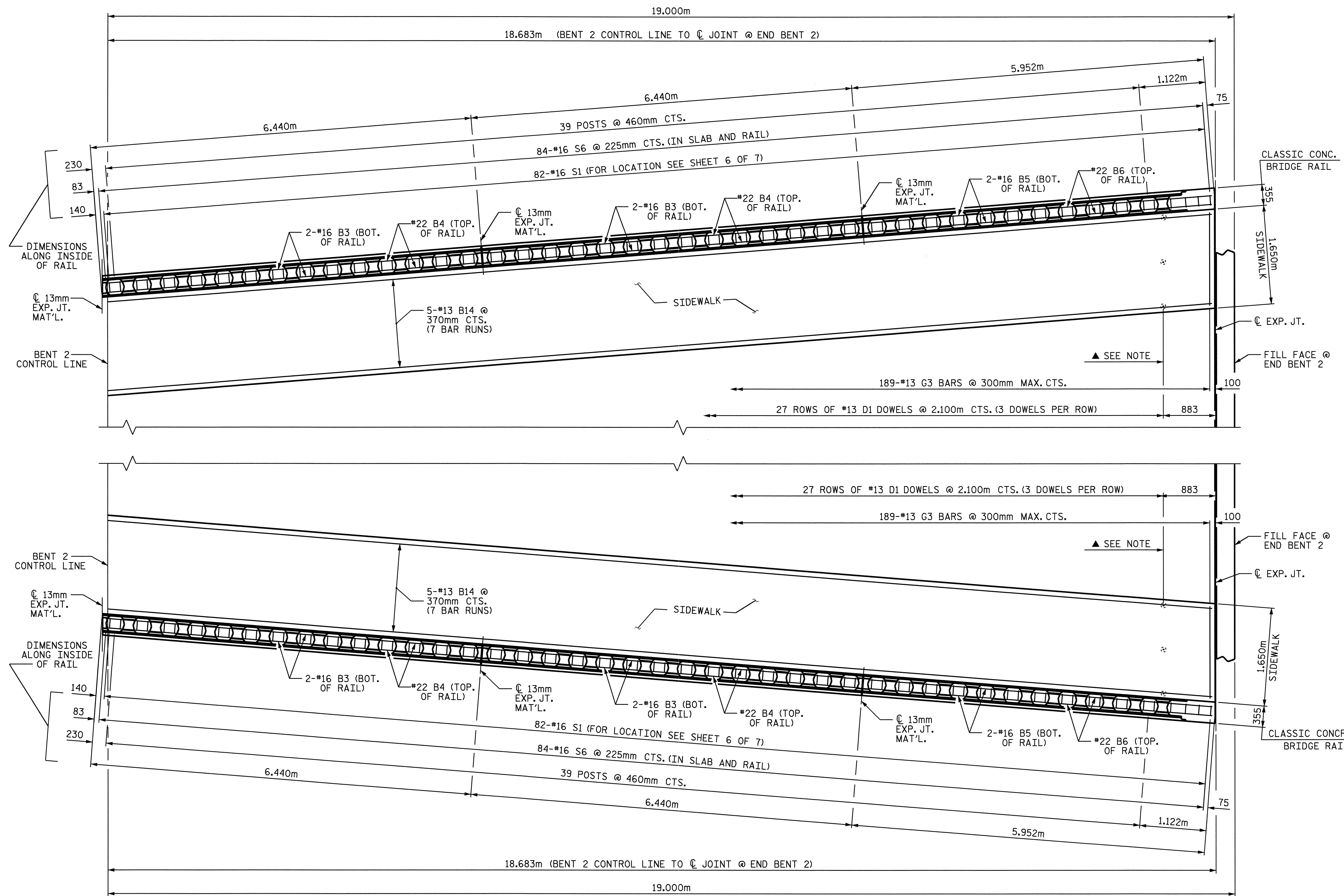
PLAN OF SPAN C
