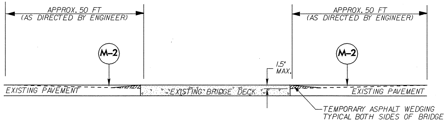
DETAIL NO. 2 MILLING BRIDGE DECK AND APPROACHES SEE CHART BELOW FOR EXISTING BRIDGE PAVING INSTRUCTIONS
