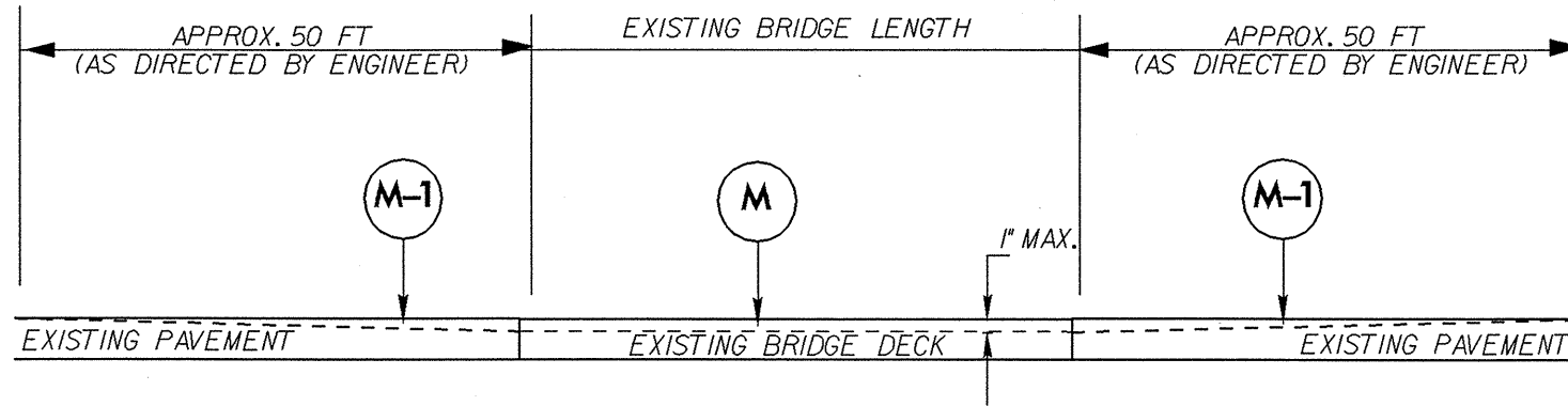
DETAIL NO. 1 MILLING BRIDGE DECK AND APPROACHES SEE CHART BELOW FOR EXISTING BRIDGE PAVING INSTRUCTIONS
