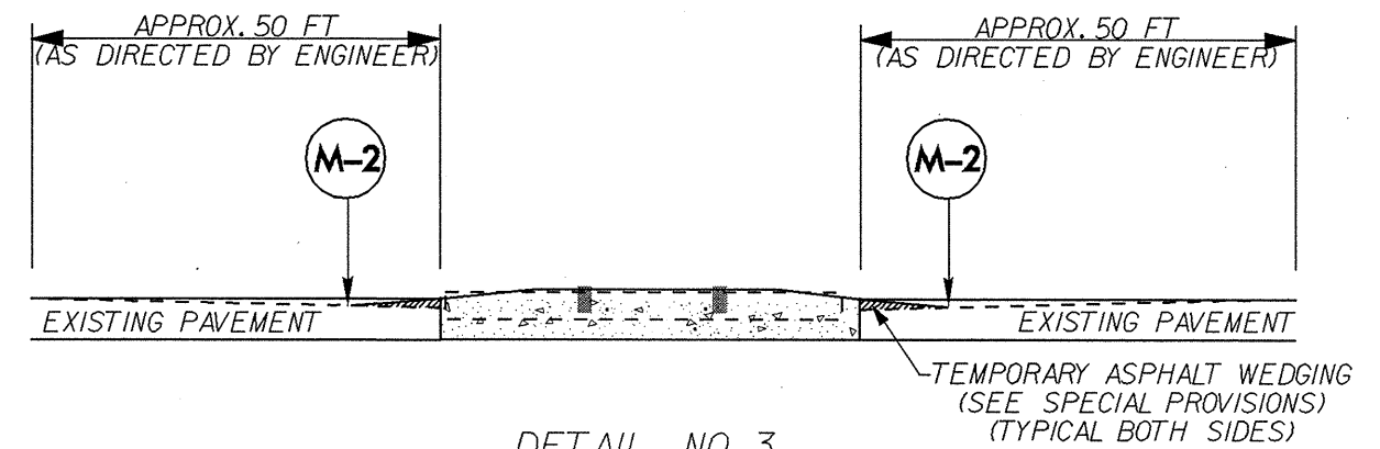
DETAIL NO. 3 MILLING RAILROAD CROSSING APPROACH
