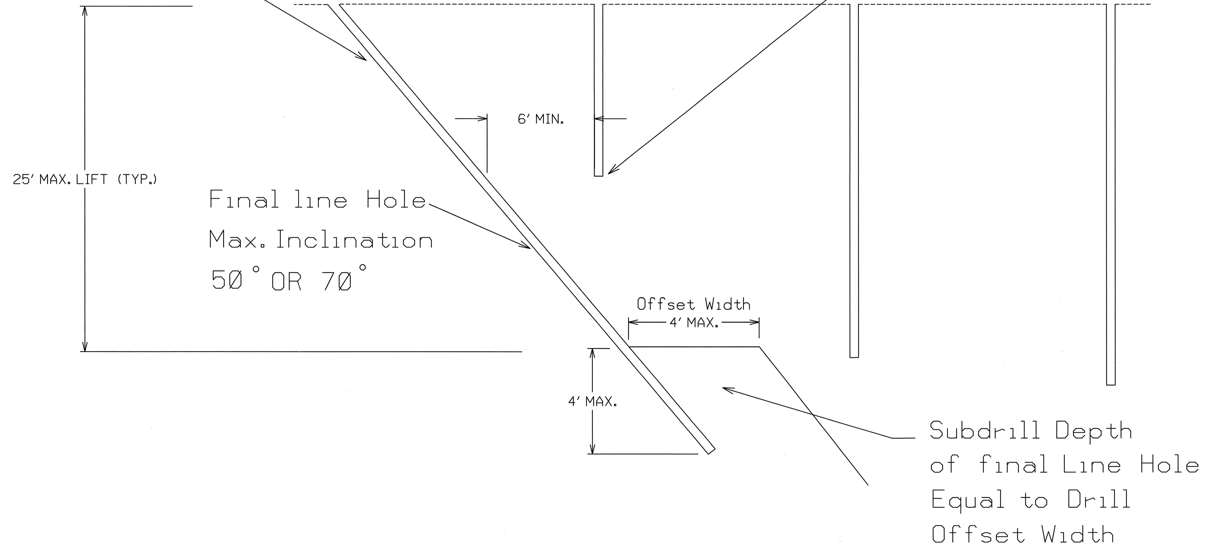
TYPICAL BLASTHOLE LAYOUT FOR 1/2:1 AND 1:1 SLOPE
