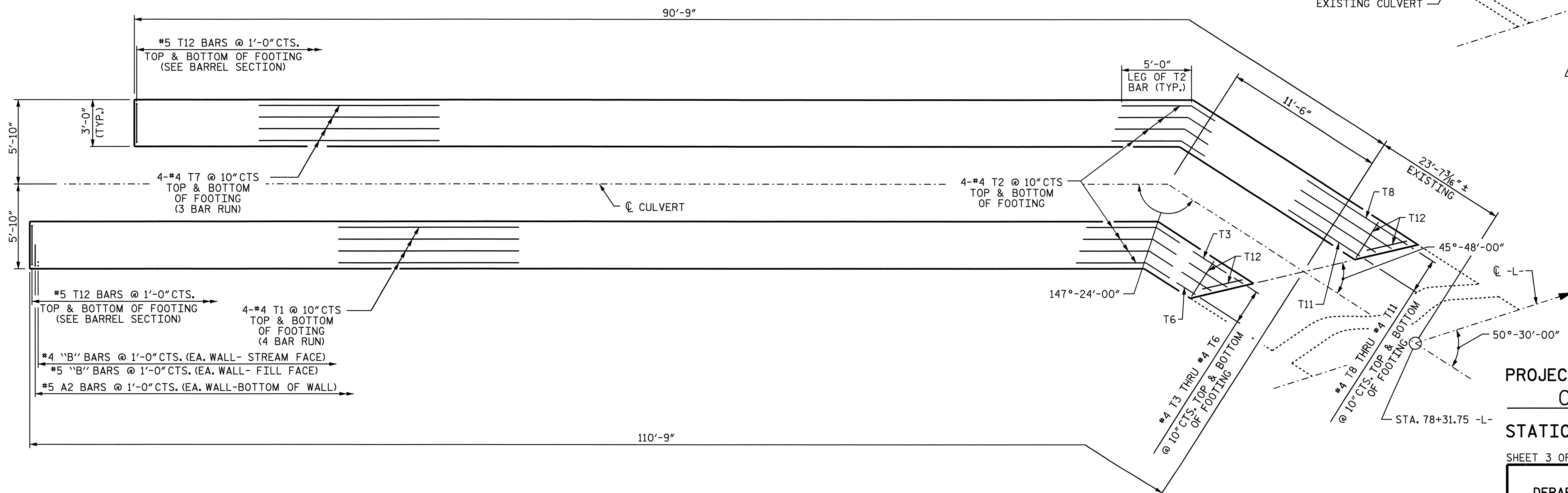
PLAN OF FOOTING
