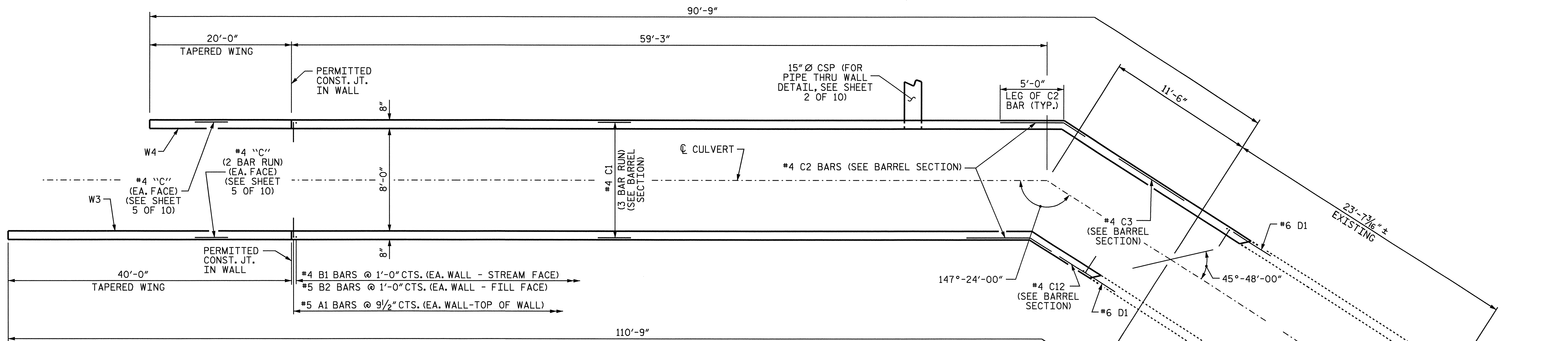
PLAN OF WALL
