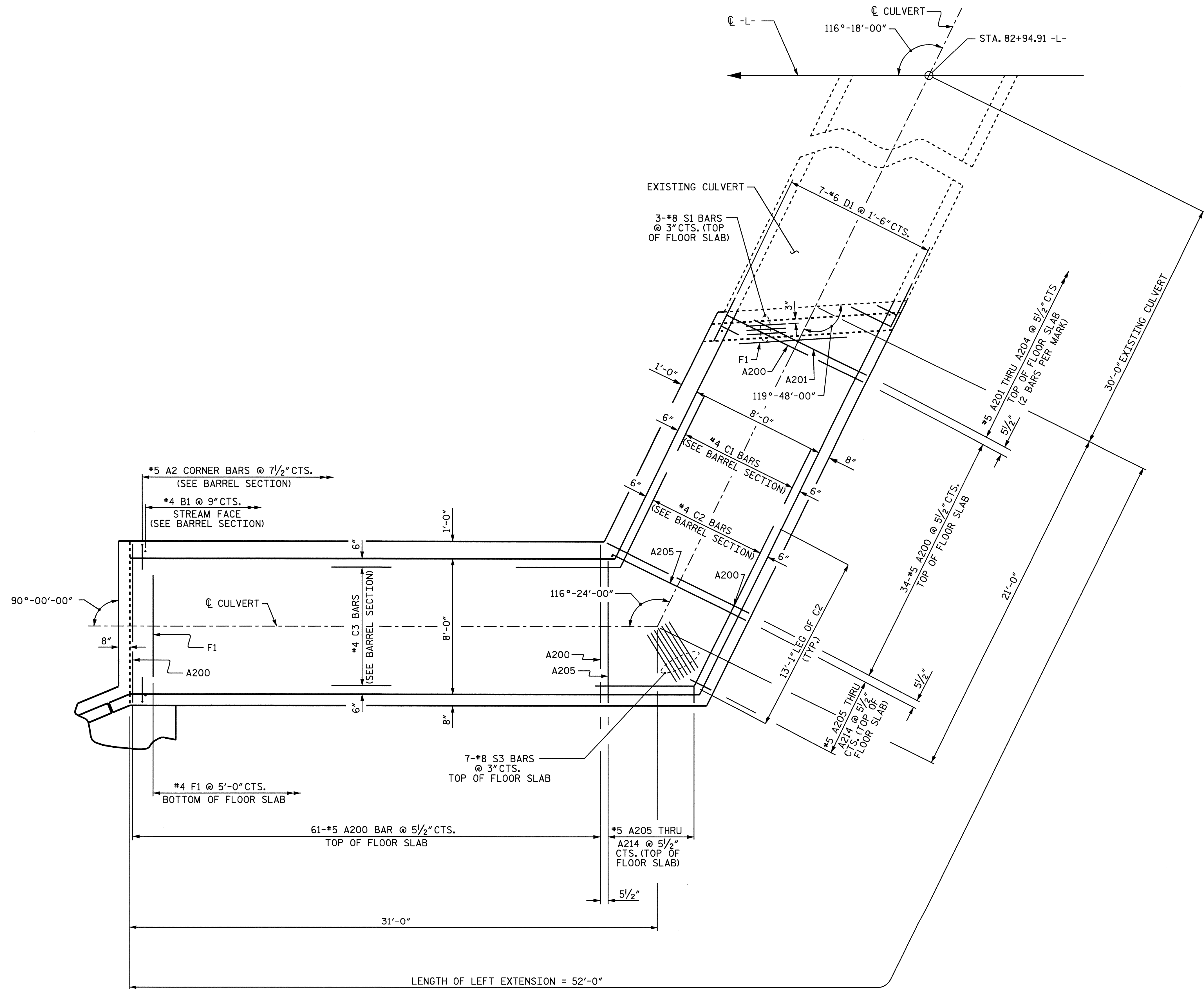
PLAN OF FLOOR SLAB
