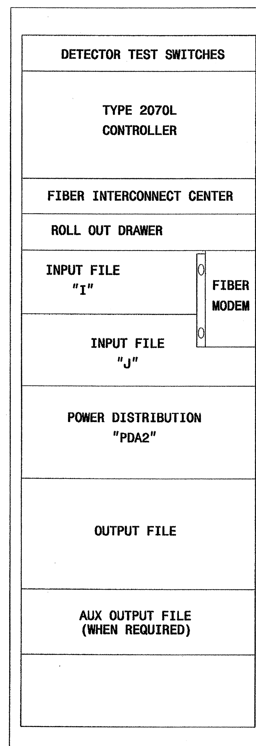
332A CABINET
