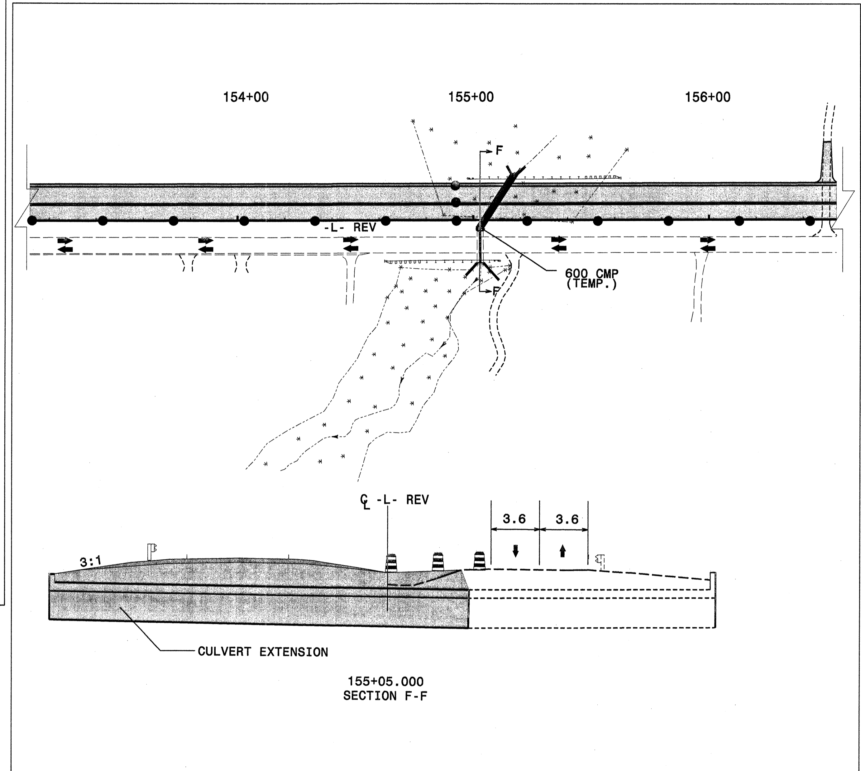
DETAIL 11
