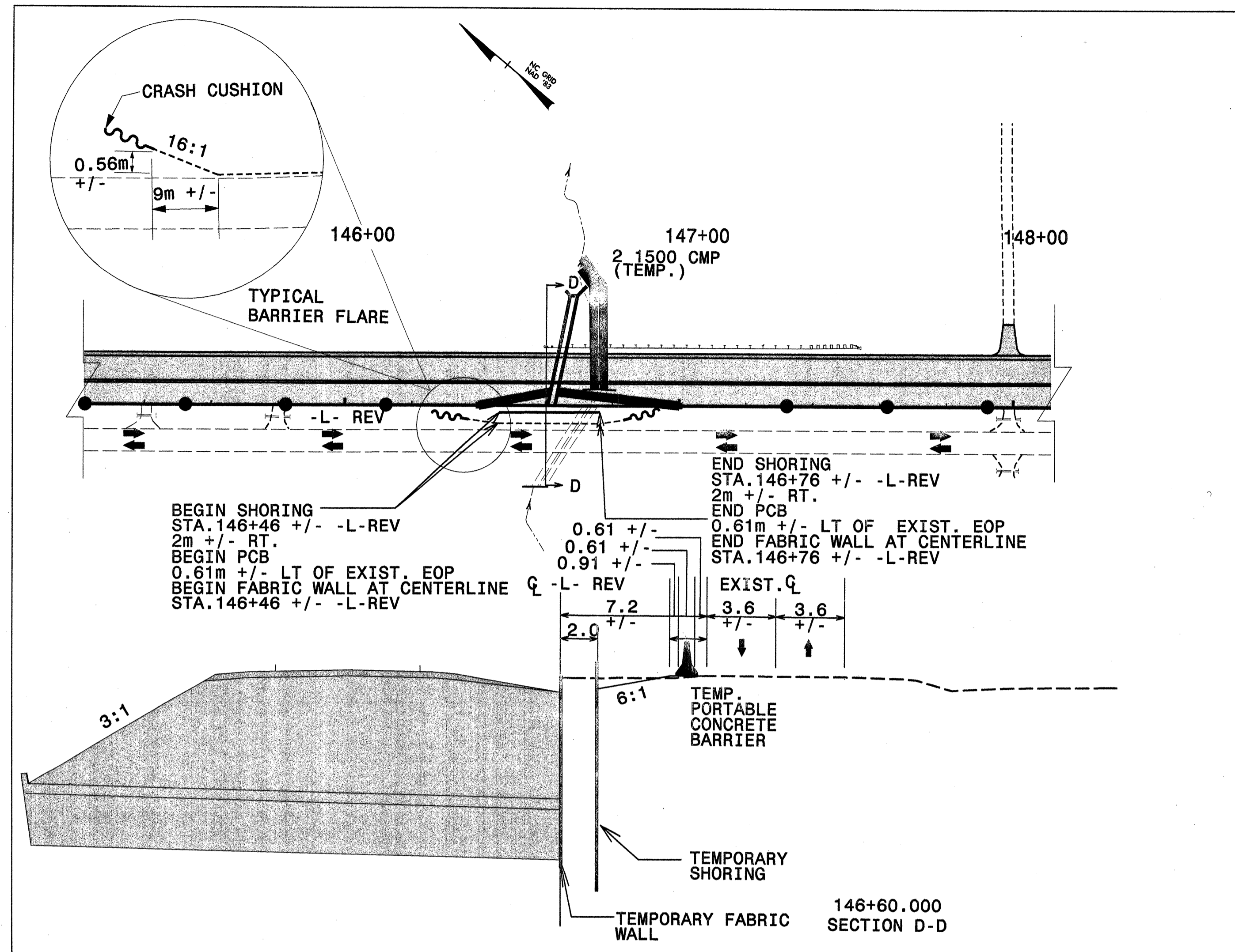
DETAIL 10
