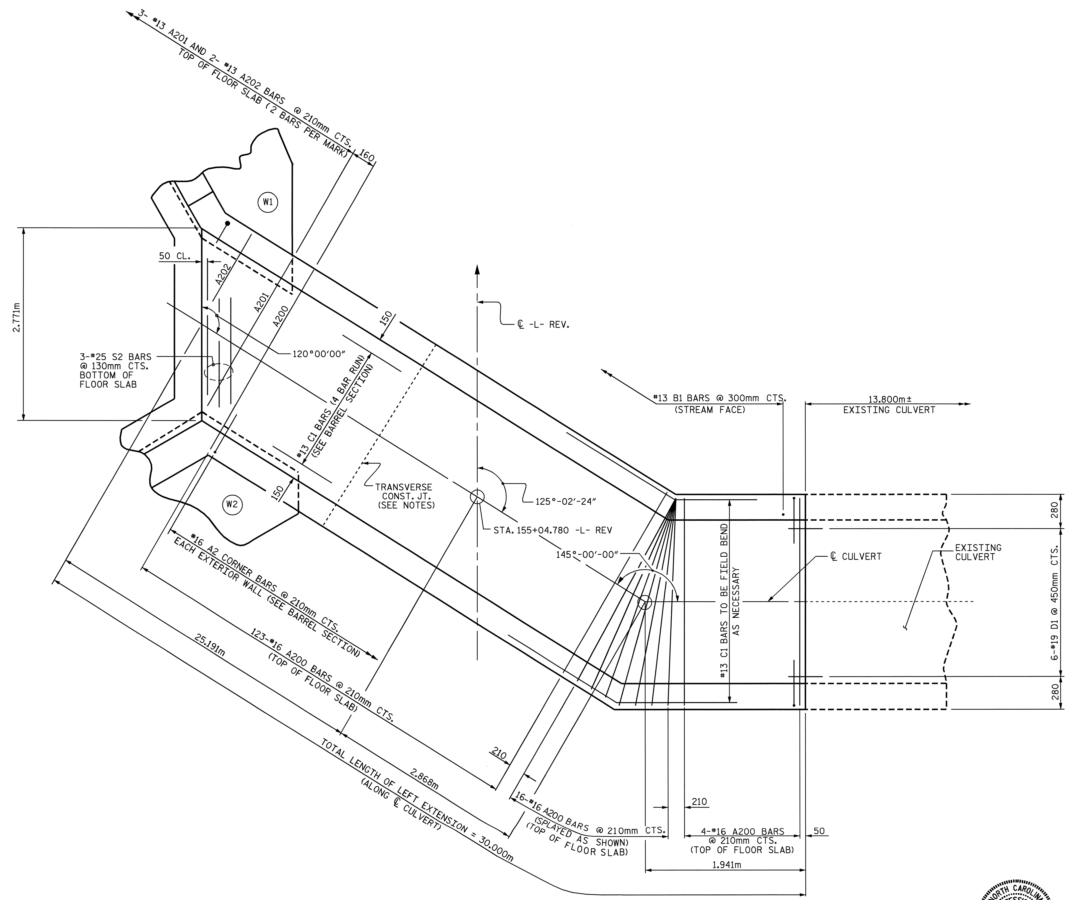
PLAN - FLOOR SLAB
