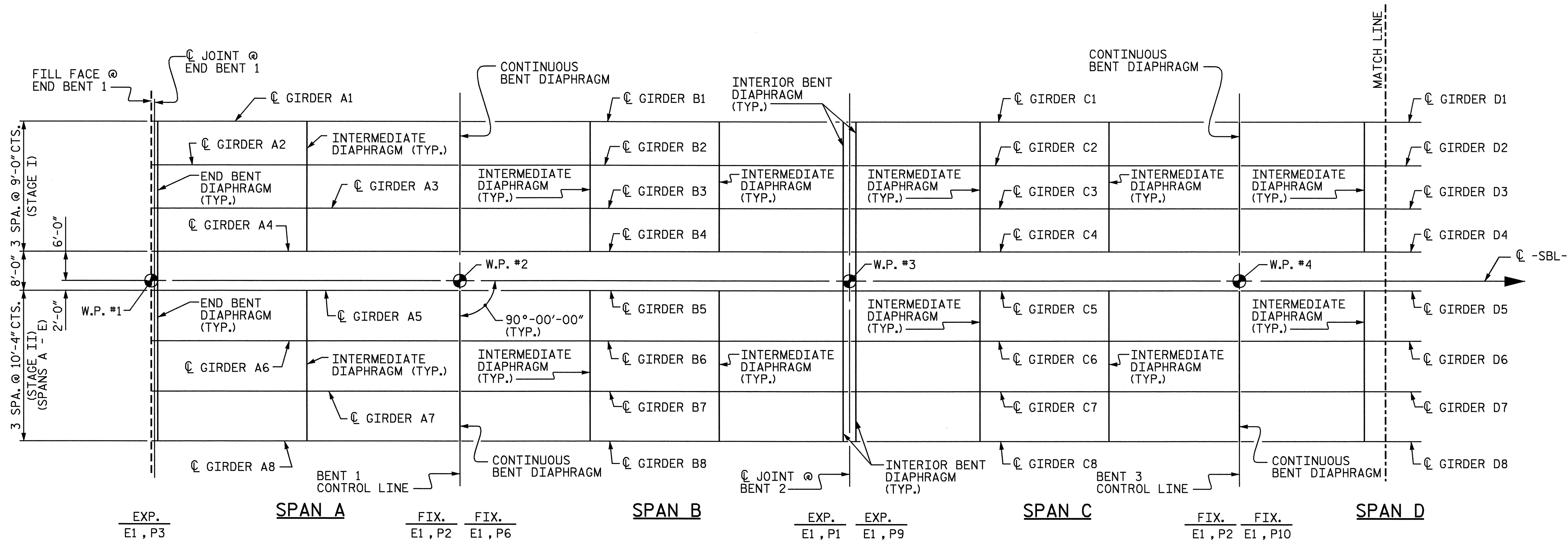
PARTIAL GIRDER LAYOUT SHOWING SPANS A THROUGH D
