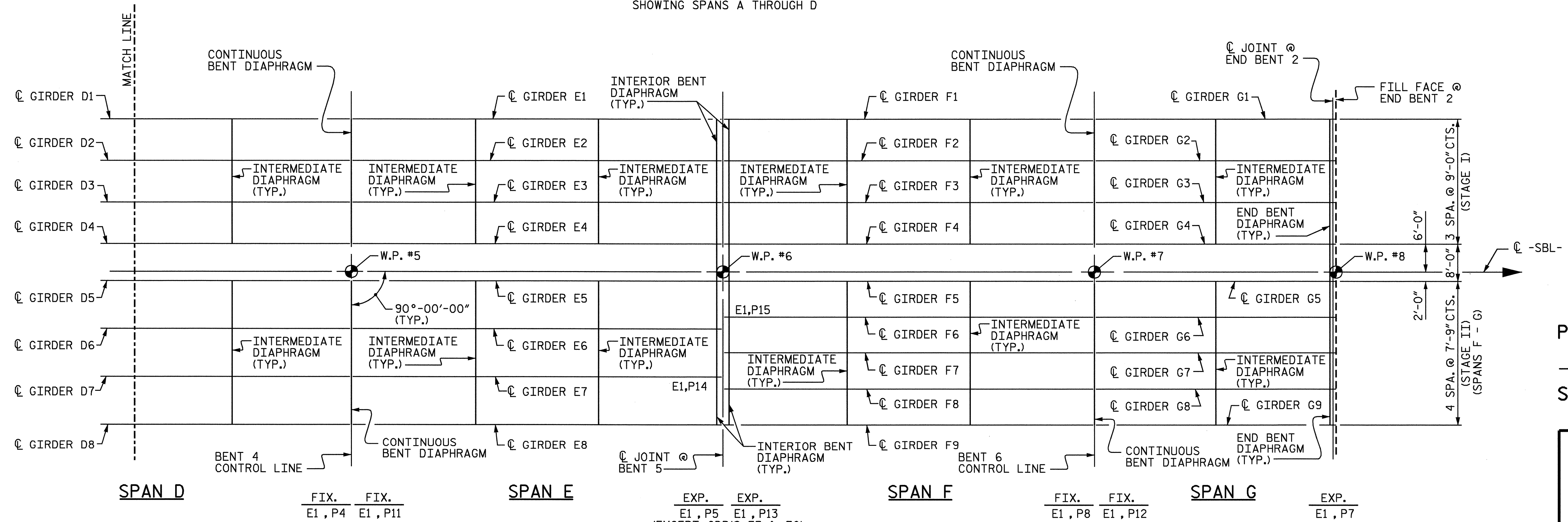
PARTIAL GIRDER LAYOUT SHOWING SPANS D THROUGH G
