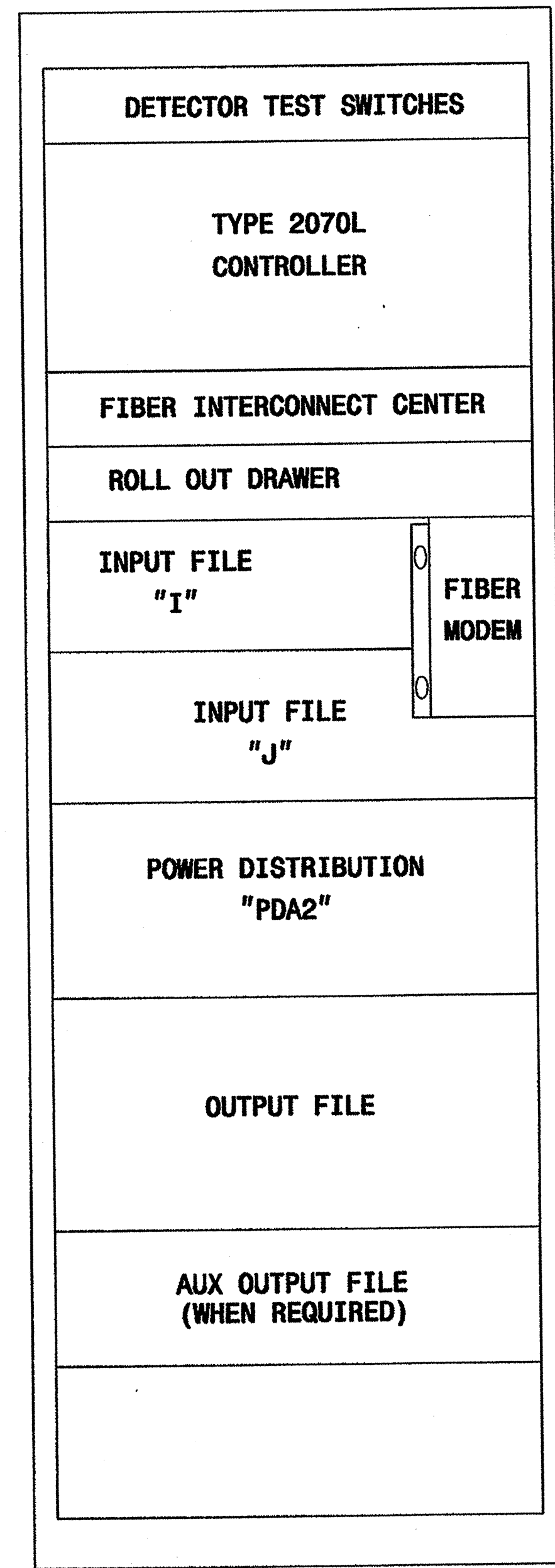
332A CABINET REAR VIEW
