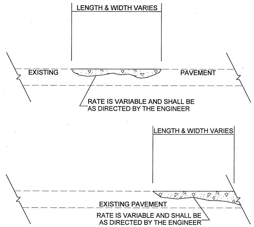
ASPHALT CONCRETE SURFACE COURSE (LEVELING COURSE)
