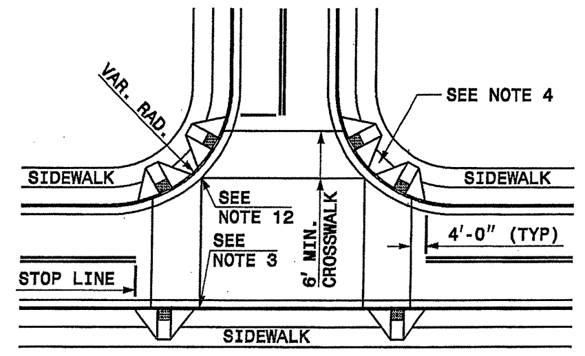
DETAIL SHOWING TYPICAL LOCATION OF WHEELCHAIR RAMPS, PEDESTRIAN CROSSWALKS AND STOP LINES FOR TEE INTERSECTIONS
