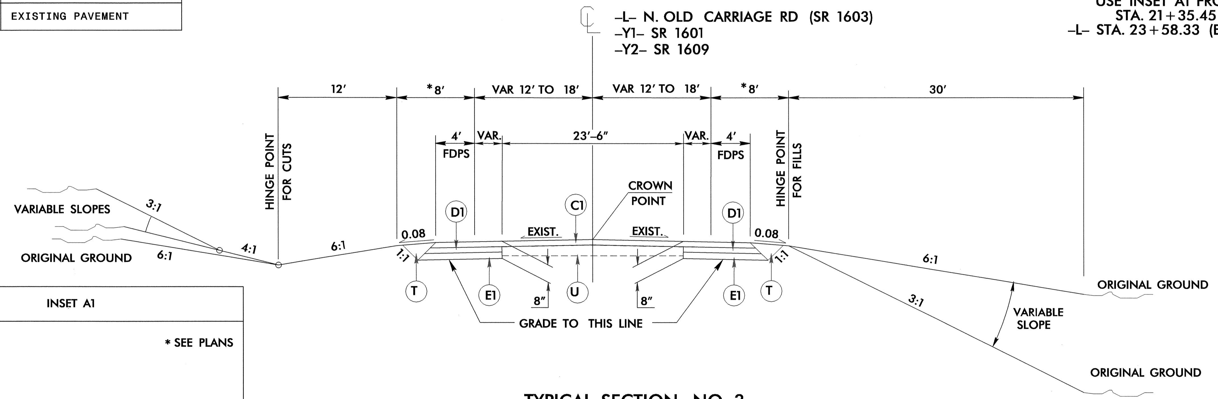
TYPICAL SECTION NO. 3
