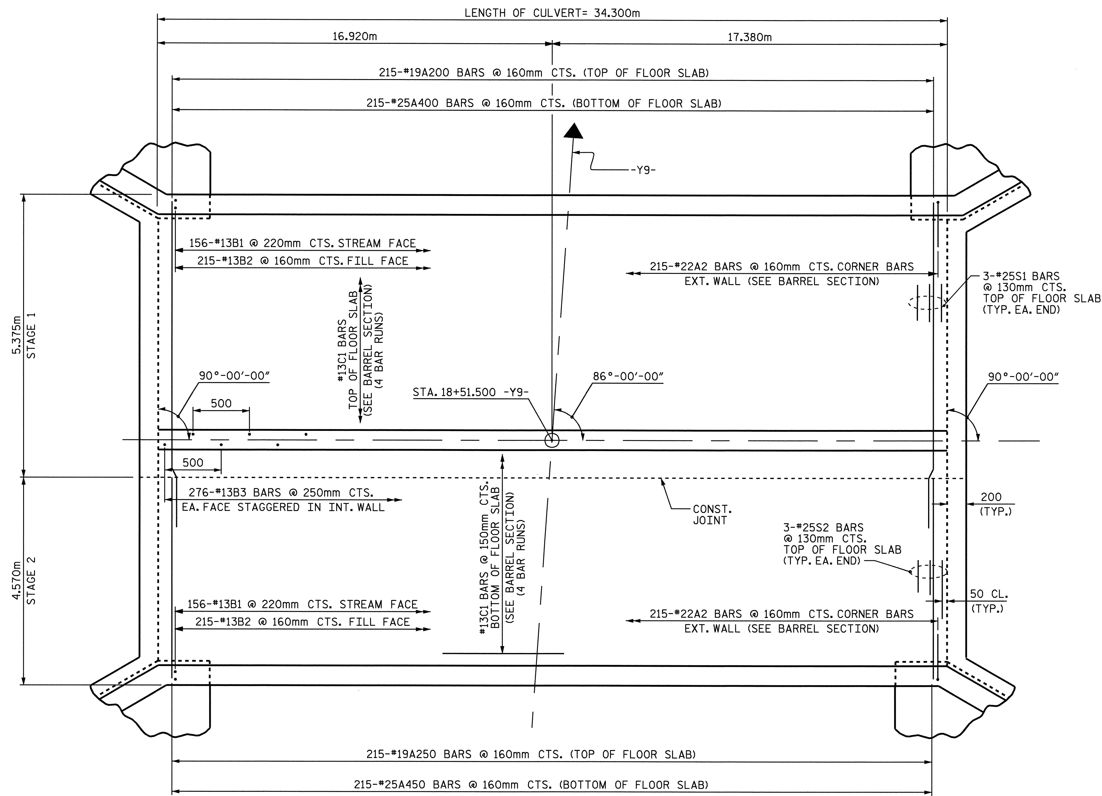
PLAN-FLOOR SLAB
